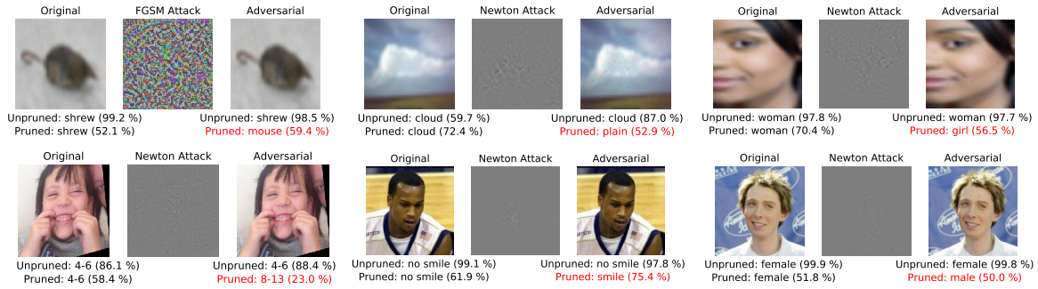
Figure 4: Example adversarial attacks that have fooled the pruned net, but not the original unpruned one
