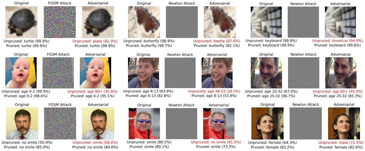
Figure 3: Example adversarial attacks that have fooled the original unpruned net, but not our pruned one
