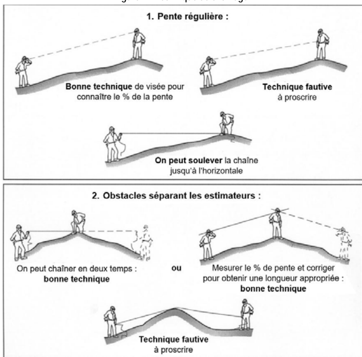
Figure A1 Technique de chaînage
