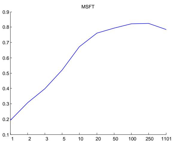
Figure E.4: Average weekly betas of individual stocks against the frequency (in ticks) used in their calculation. Data year 2006.
