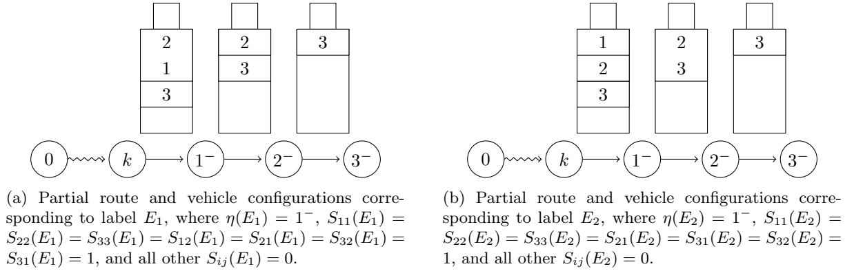
Figure 5: Possible extension of labels E_1 and E_2 , where items 1 and 2 are at the same level for label E_1 , but at different levels for label E_2 . The extension might be feasible for label E_2 but not for label E_1 .
