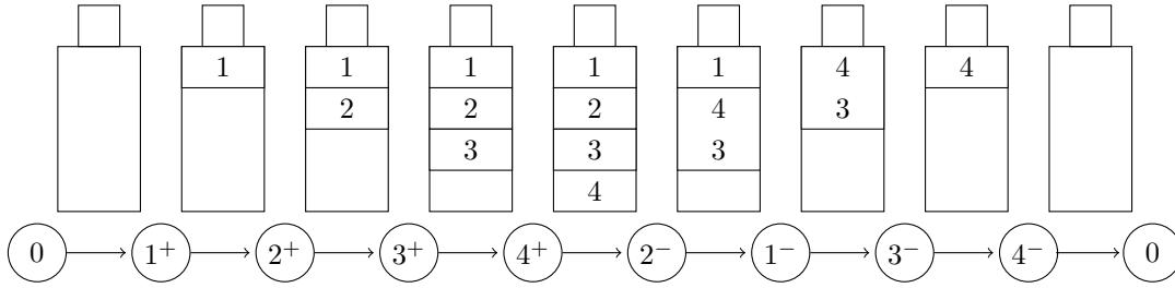
Figure 2: Example of a route with its corresponding vehicle configuration under policy 1. There is no separation line between items at the same level.
