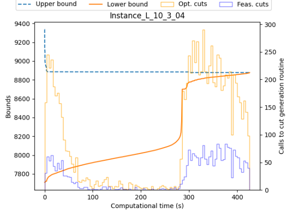
(b) Example 1 with Benders-3 (10 customers).
