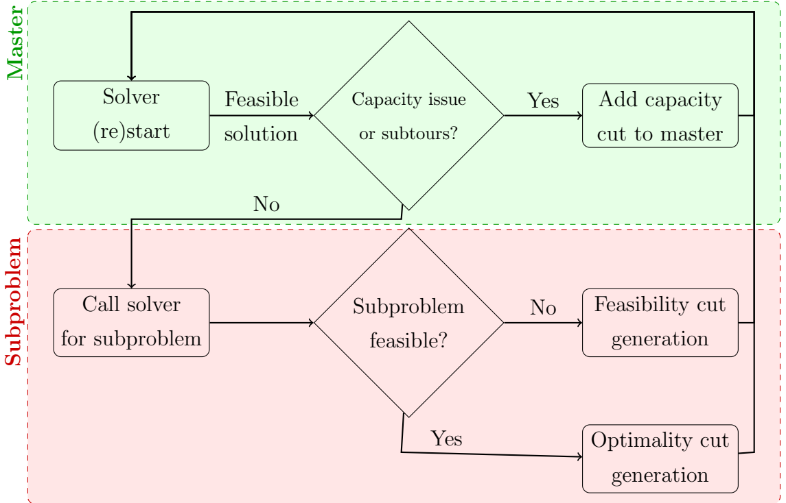
Figure 1: Schematic representation of the decomposition algorithm.
