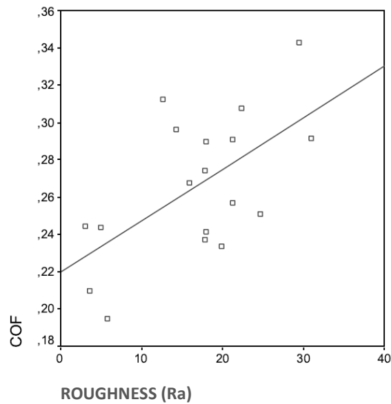
Figure 4 Regression between the COF on ice ( -12^{\circ}\text{C} ) and sole roughness (adapted from Gao et al., 2004).
