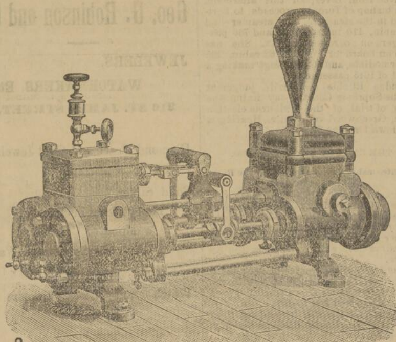
WORTHINGTON PATTERN DUPLEX STEAM PUMP.
