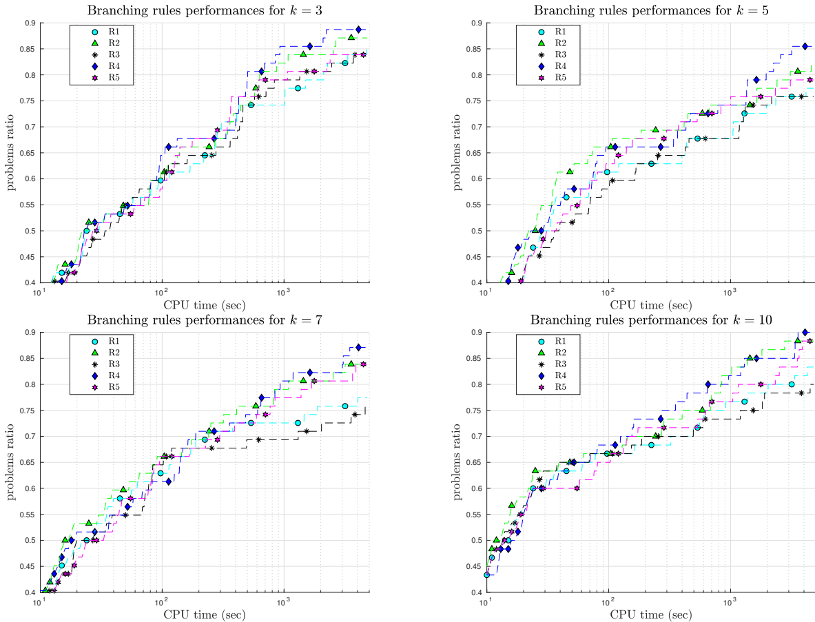
Figure 4: Performance profiles of five branching rules, for the instances of SET A and for k \in \{3, 5, 7, 10\} .
