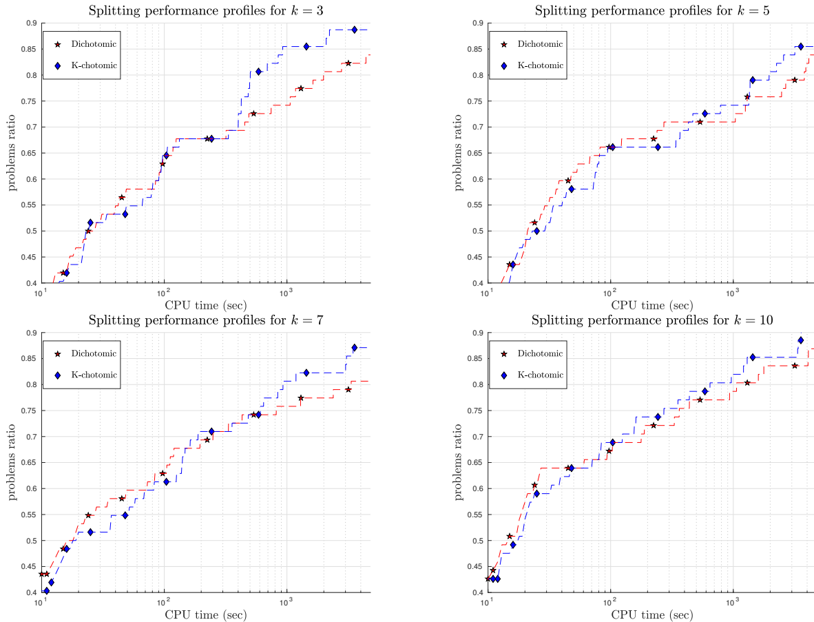
Figure 3: Performance profiles of dichotomic and k -chotomic strategies, for the instances of SET A and for k \in \{3, 5, 7, 10\} .
