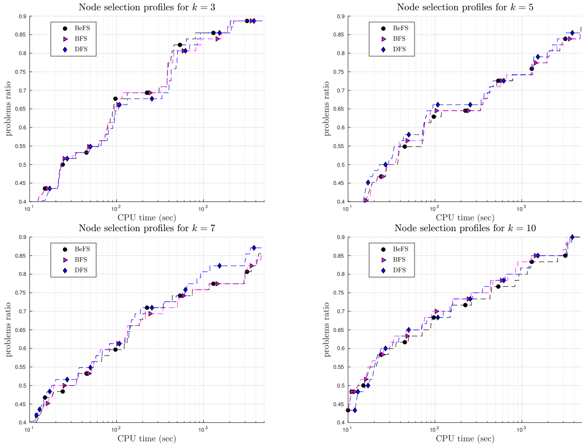
Figure 5: Performance profiles of three strategies of node selection: BeFS, BrFS, and DFS; for k \in \{3, 5, 7, 10\} and for the instances of SET A.
