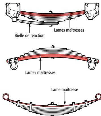
FIGURE 52 | Lames maîtresses
