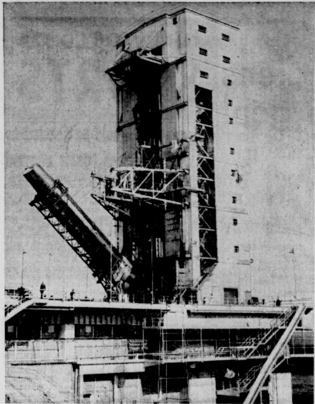
AUSTRALIA ENTERS SPACE AGE — A British Blue Streak rocket is raised on its launching pad in preliminary tests for a space shot that will put Australia's Woomera rocket range into the major league of world space research centres. The 100-ton vehicle will be fired
