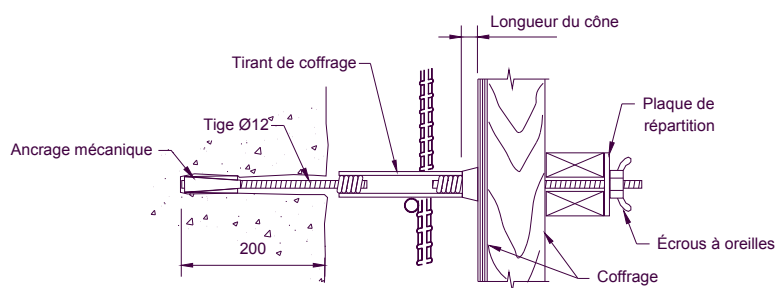
Figure 4.3-6 Tirant type
