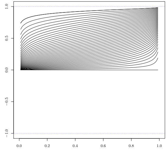
(b) Tail dependence function \bar{\chi}(u) , u \in (0, 1)
