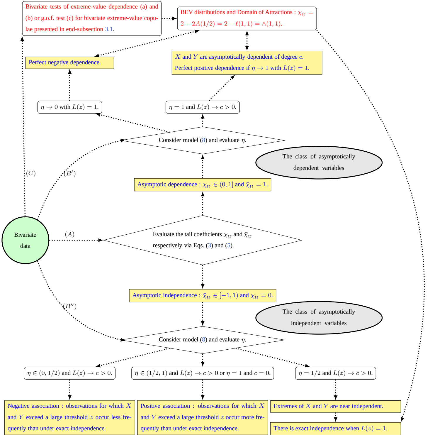
Figure 2: Diagram of the study of the tail dependence in bivariate frequency analysis. The circle denotes the starting point. We can follow the path (A), (B'), (B'') or (C), however we recommend to follow the path (A).
