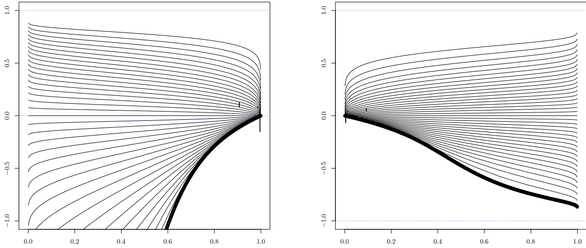
(a) Tail dependence function \chi(u) , u \in (0, 1)
