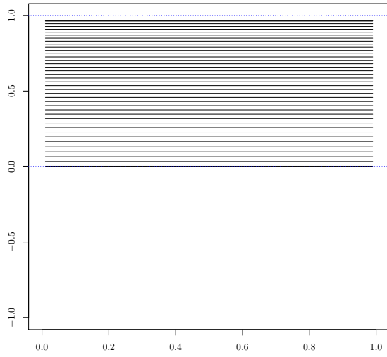
(a) Tail dependence function \chi(u) , u \in (0, 1)
