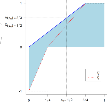
Figure 4: \bar{V}(p)
