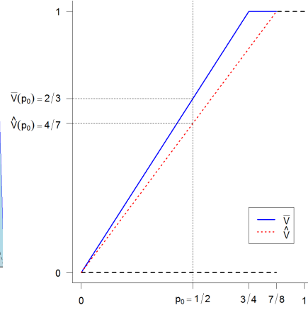
Figure 9: \bar{V}(p) .
