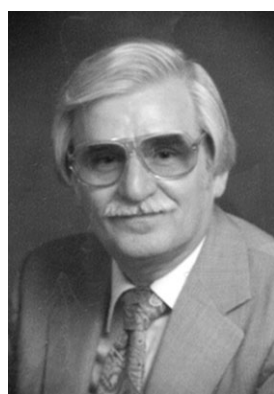
ROGER LETELLIER
