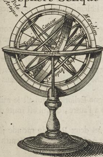
Sphere Oblique
