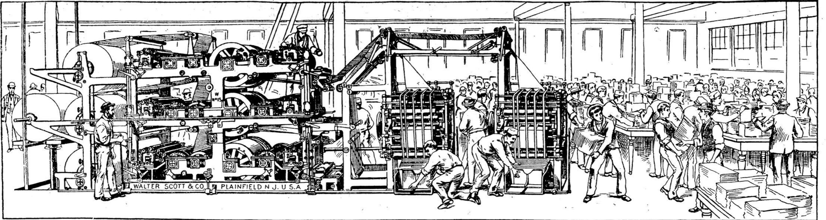
THE NEW "STAR" PRESS AS SEEN IN MOTION IN THE "STAR" PRESSROOM, SPEED, 48,000 PERFECTED PAPERS PER HOUR. BUILT BY WALTER SCOTT & CO., NEW YORK AND PLAINFIELD.
