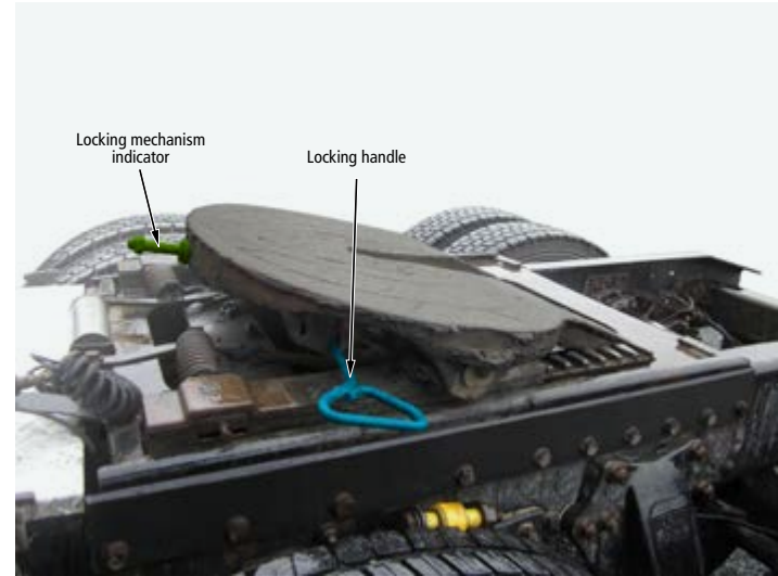
FIGURE 12 | Fifth wheel (locking mechanism indicator and locking handle)
