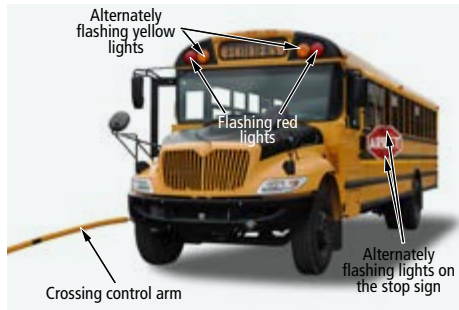
FIGURE 71 | School bus
