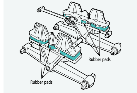
FIGURE 51 | Rubber pad suspension
