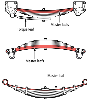
FIGURE 52 | Master leaves
