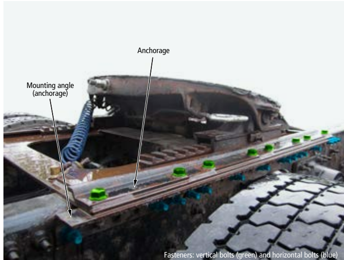
FIGURE 6 | Fifth wheel fasteners
