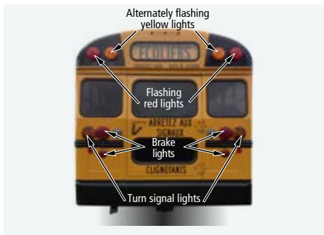
FIGURE 33 | Rear lights of a school bus
