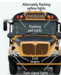
FIGURE 32 | Headlights and front lights of a school bus
