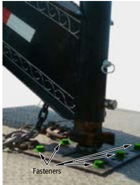
FIGURE 16 | Gooseneck coupling device
