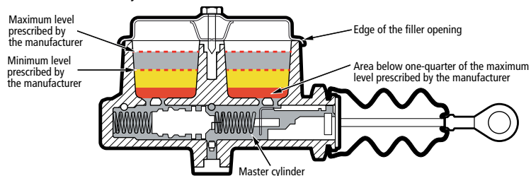
FIGURE 58 | Master cylinder reservoir with indicators from the manufacturer
