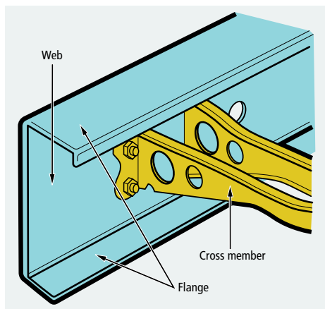
FIGURE 20 | Side rail and cross member
