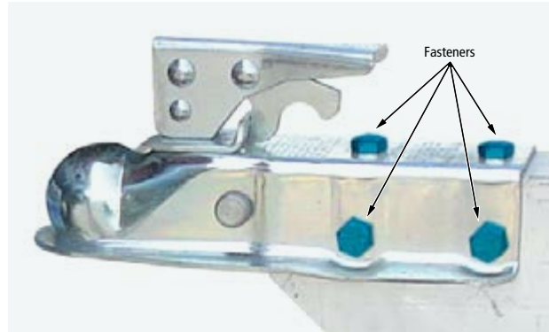
FIGURE 17 | Ball and hitch coupling device
