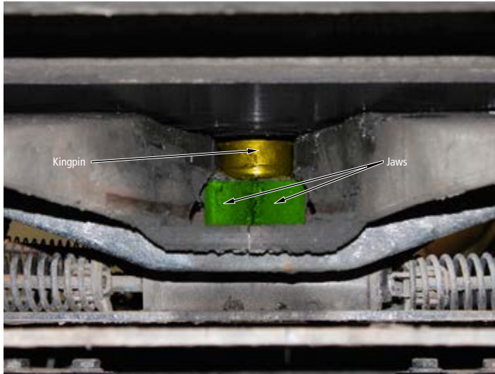
FIGURE 11 | Fifth wheel jaws
