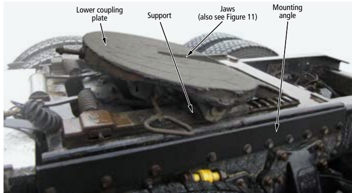
FIGURE 9 | Components of the fifth wheel
