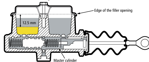
FIGURE 59 | Master cylinder reservoir without indicators from the manufacturer
