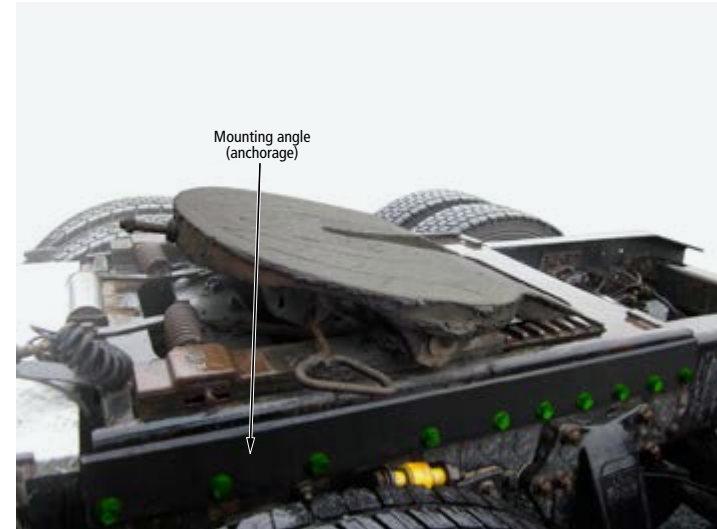
FIGURE 7 | Fifth wheel fasteners
