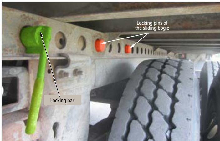
FIGURE 21 | Sliding bogie
