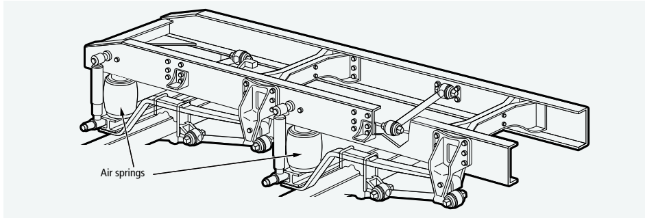
FIGURE 50 | Pneumatic suspension
