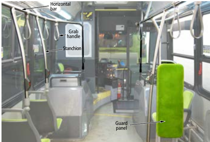
FIGURE 72 | Stanchions, horizontal bars, grab handles and guard panel
