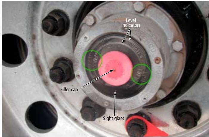
FIGURE 46 | Wheel hub sight glass
