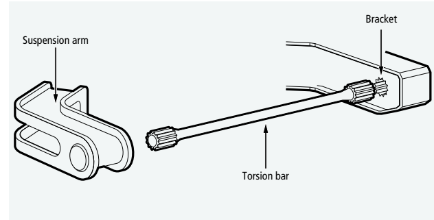
FIGURE 49 | Torsion bar
