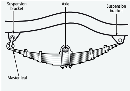
FIGURE 47 | Leaf spring
