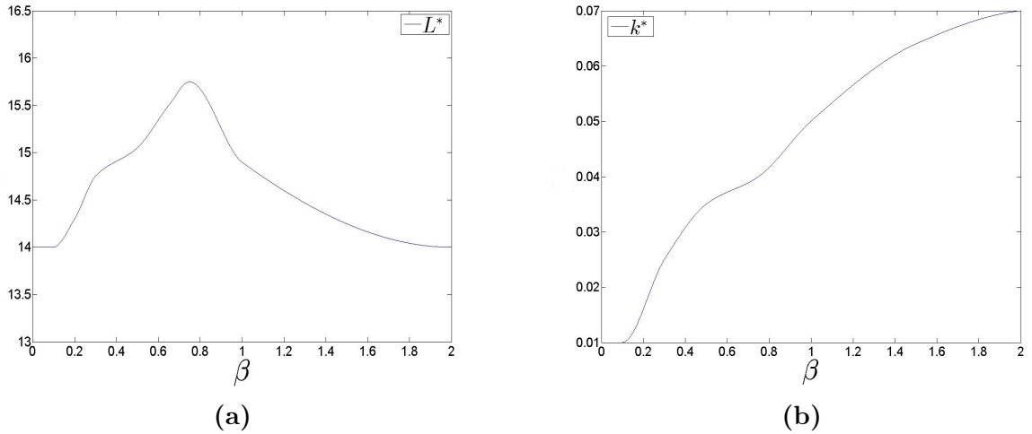
Figure 2: Optimal Investment Threshold L^* (Figure 2a) and Optimal Mitigation Investment Fraction k^* (Figure 2b), plotted against Volatility \beta , for D = 50
