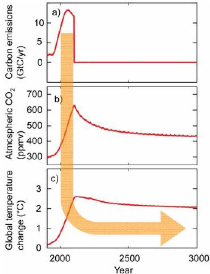
Figure 10: Decay Rate of Temperature as a Function of Emission Reductions
