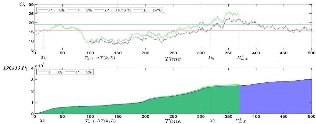
Figure 4: Impacts of Mitigation vs. Adaptation only on the Temperature Process and on the Sum of Discounted Future Disposable GDPs, for \beta = 0.75^\circ C
