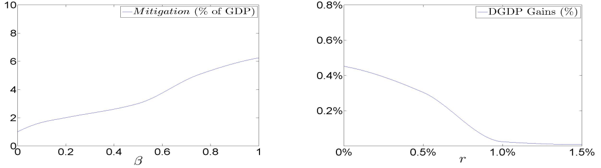
(a) Mitigation Efforts, as fraction of GDP, plotted against volatility \beta (b) Cumulative DGDP Gains (%) of Mitigation vs. Adaptation only, as function of r and for \beta = 0.75^\circ C
