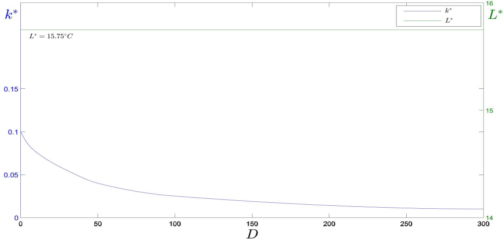
Figure 5: Optimal Mitigation Investment Fraction k^* and Optimal Investment Threshold L^* , plotted against different values of the Parisian Window D , for volatility \beta = 0.75^\circ C
