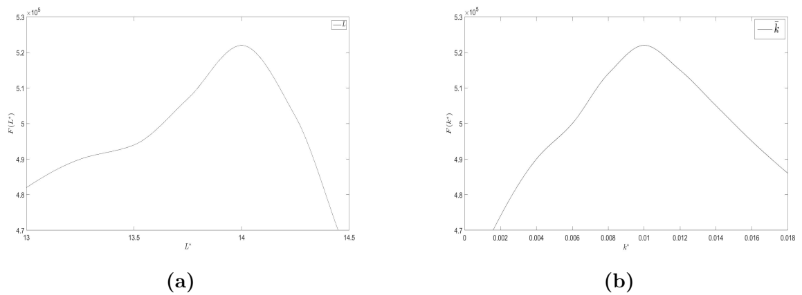
Figure 9: Maximum of the Function f , for \beta = 0^\circ C , plotted against the Optimal Investment Threshold L^* , for k^* = 1\% , and against the Optimal Mitigation Investment Fraction k^* , for L^* = 14^\circ C .
