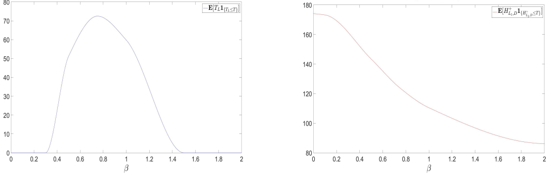
(a) Expected Date T_L plotted against Volatility \beta , for D = 50 (b) Expected Date of the Environmental Catastrophe H_{L_1, D}^+ plotted against Volatility \beta for D = 50
