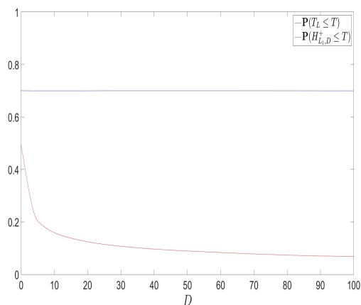
(b) Probability of T_L \leq T and Probability of H_{L_1, D}^+ \leq T , plotted against different lengths of the Parisian Window D , for \beta = 0.75^\circ C
