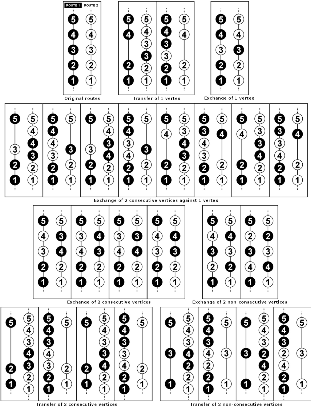
Figure 1. The tested 2-interchange moves.
