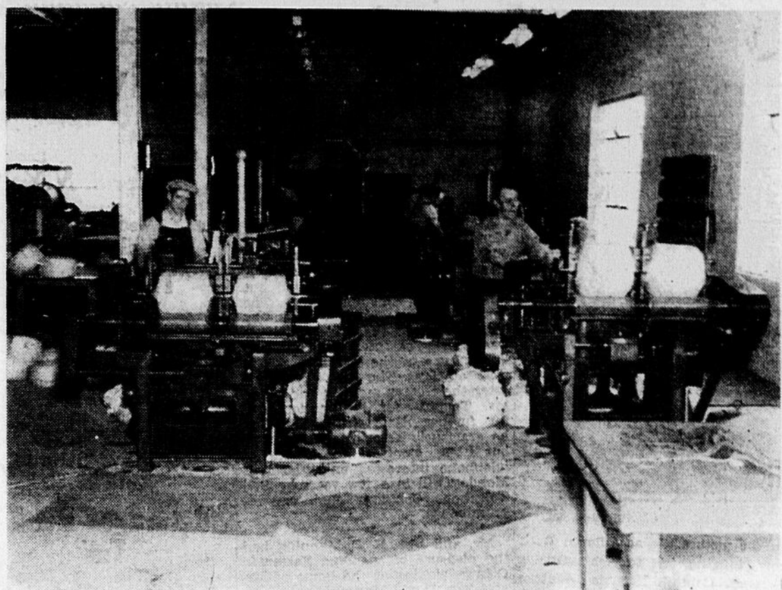
GILLING MACHINES —On the machines in the above photograph, the wool tops are wound into spools of sufficient size to suit the dye kettles. This process is known as "gilling". It is the first process after the tops are received.
