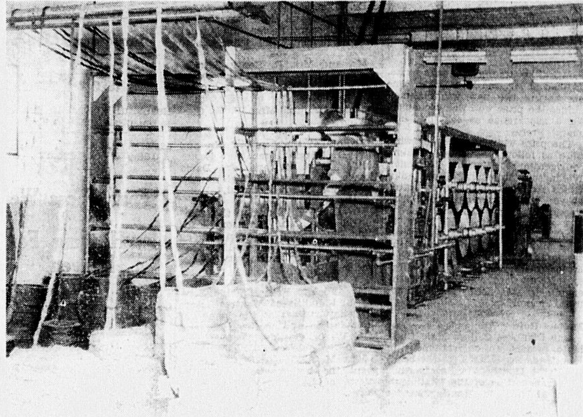
WASHING AND DRYING —After the tops have been dyed, they are placed on the machine above and first go through a bath of detergents and clear water which thoroughly rinses them. They are immediately wound onto the cylinders that can be seen and on this are dried by the heat in the cylinders. At the far end of the machine they are again gilled and come off the machine in spools of the color of the dye. Later they are put onto the gilling machine again where the wool is blended ready for spinning and weaving at the textile mill.
