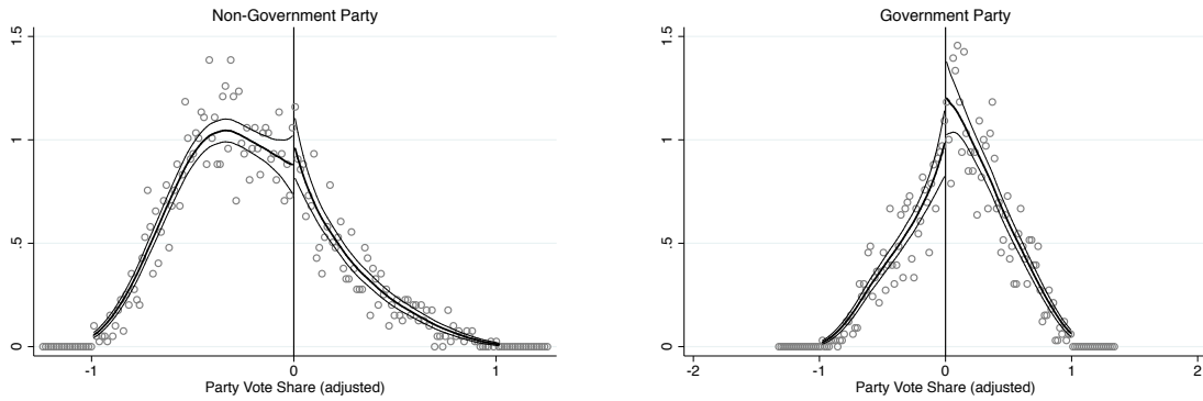
Figure A.2: Density Plot - McCrary Test by Subsample
