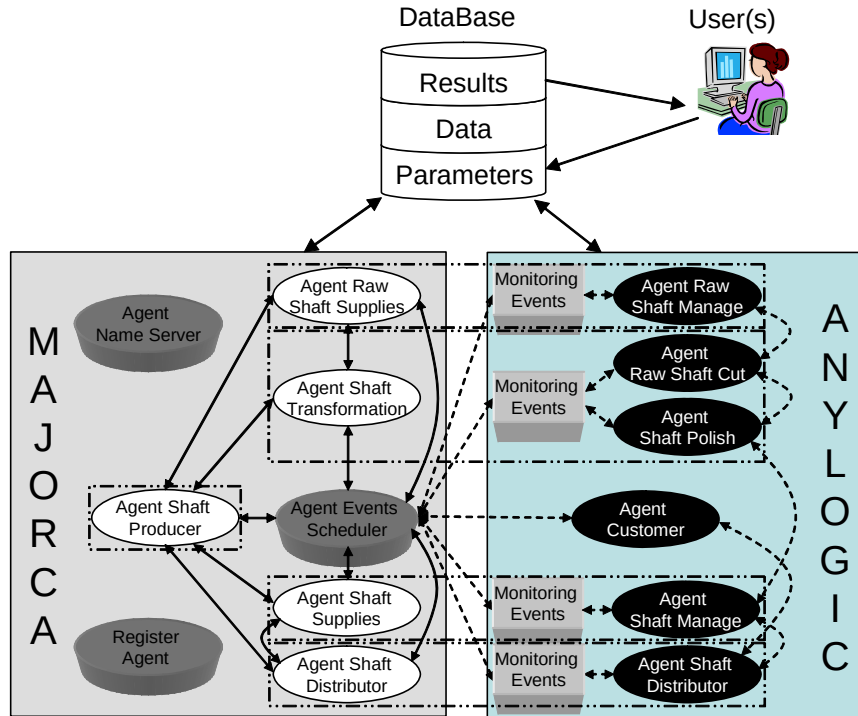
Fig. 17 : An implemented multi-agent platform
