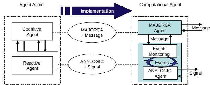
Fig. 16 : The "Computational Agent" architecture
