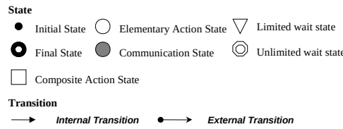
Fig. 11 : Agents Behaviour Representation (ABR) formalism [53]
