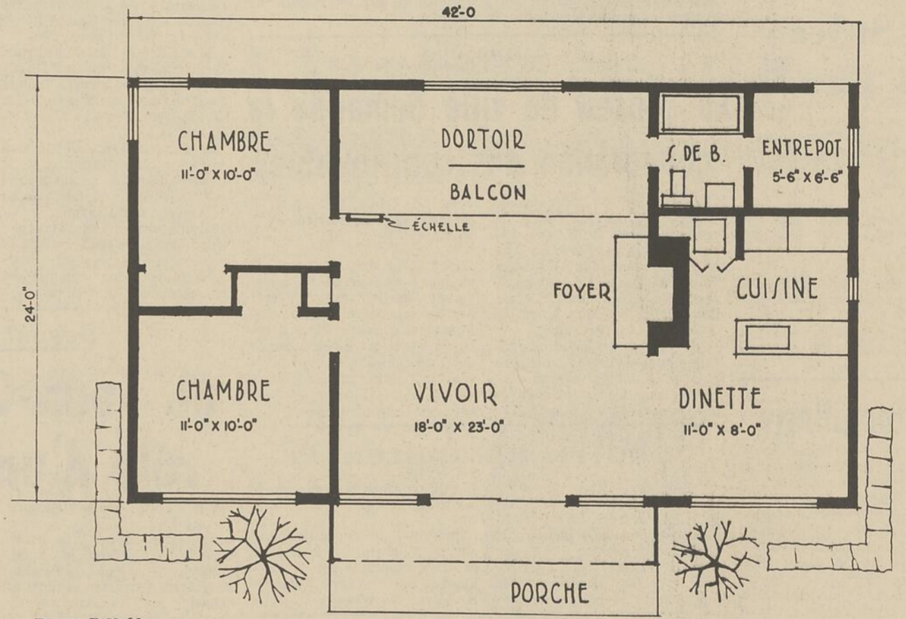
PLAN P-H-603.
