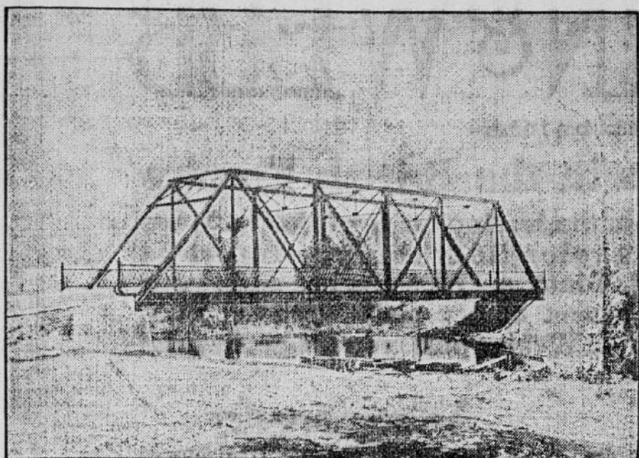
One of Our Bridges Erected Near Sutton, Quebec
