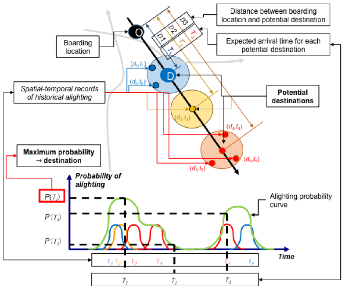
Figure 2. An illustration of the method to determine the most probable destination based on the history of the card (from He and Trépanier 2015)
