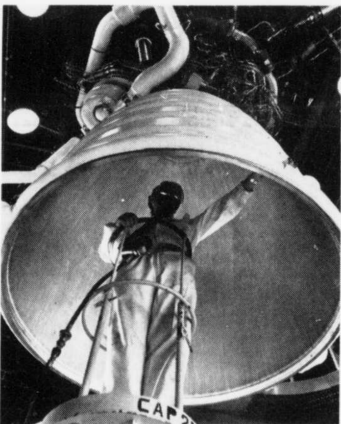
INSPECTING THE interior of the thrust chamber of an engine unit for NASA's Space Shuttle, a technician at the Rocketdyne Division of Rockwell International in Pittsburgh approves it for test firing. Three such chambers will each provide about 470,000 pounds of thrust for the shuttle transportation system.
