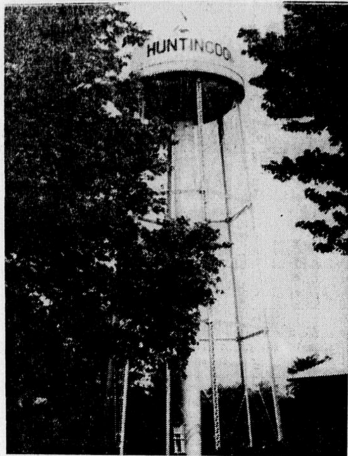
The high water tank is used only as a reserve in case of power failure or excessive demands on the water system such as the fighting of a large fire would make. Tank holds 100,000 gallons.
