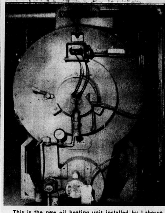
This is the new oil heating unit installed by Laberge & Lalonde (Huntingdon) which replaces an earlier coal burner. Hot air ducts travel from the furnace to all parts of the filter plant.
