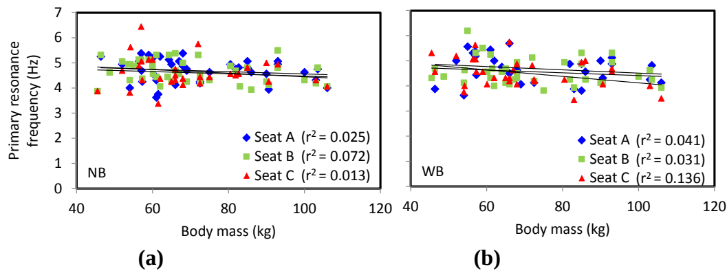
Figure 5.18: Correlations between primary resonance frequencies and body mass for the two sitting conditions and the 0.50 \text{ m/s}^2 excitation: (a) NB – without a back support; and (b) WB – with a back support (both male and female subjects included).
