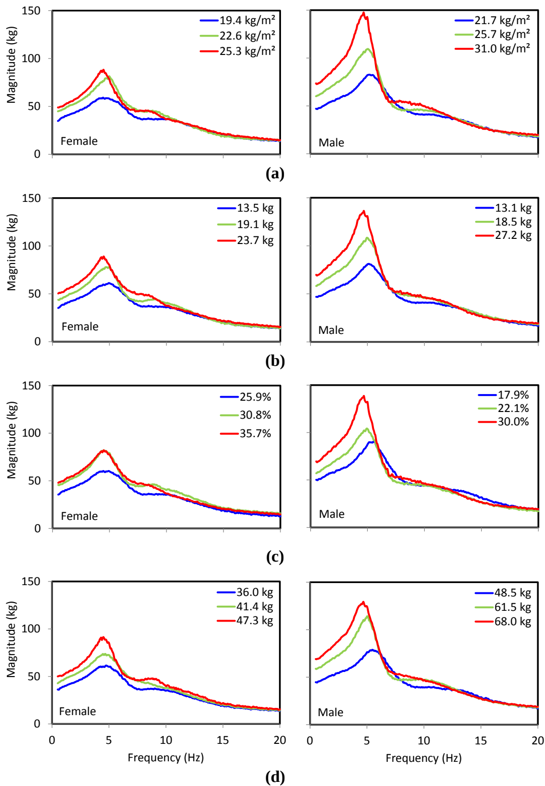
Figure 4.12: Effect of mass-related factors on the mean APMS magnitude responses of male and female subjects: (a) BMI; (b) body fat; (c) body fat percentage; and (d) lean body mass (NB posture, 0.50 m/s 2 excitation).
