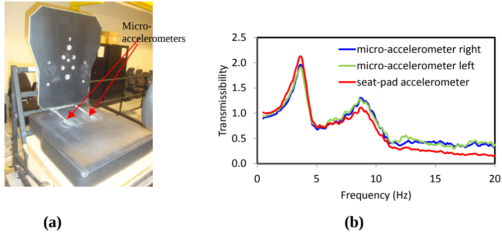
Figure 3.7: (a) Mounting of the accelerometers on an elastic seat; (b) comparisons of acceleration transmissibility measured by micro-accelerometers and standardized seat-pad-accelerometer (81 kg subject; 0.5 m/s 2 ).
