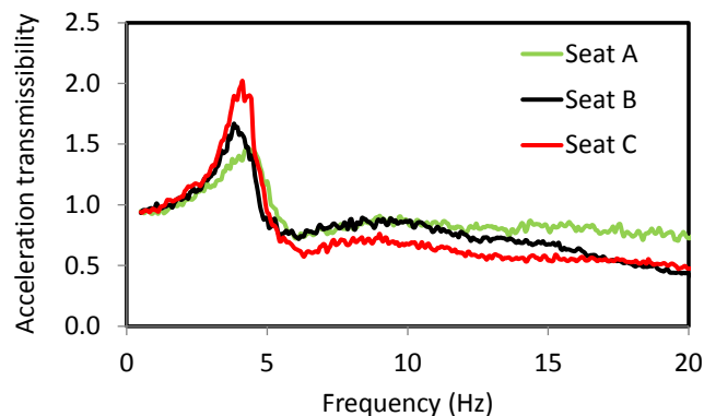
Figure 5.19: Vibration transmissibility characteristics of selected elastic seats ( 81 \text{ kg} subject; 0.50 \text{ m/s}^2 excitation at the seat cushion).
