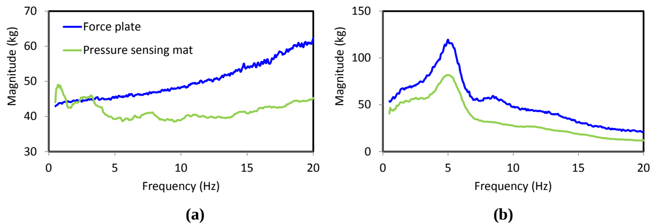
Figure 3.10: Comparisons of the APMS magnitude responses derived from the force plate and the pressure sensing mat: (a) 44 kg rigid load; and (b) 83 kg subject.
