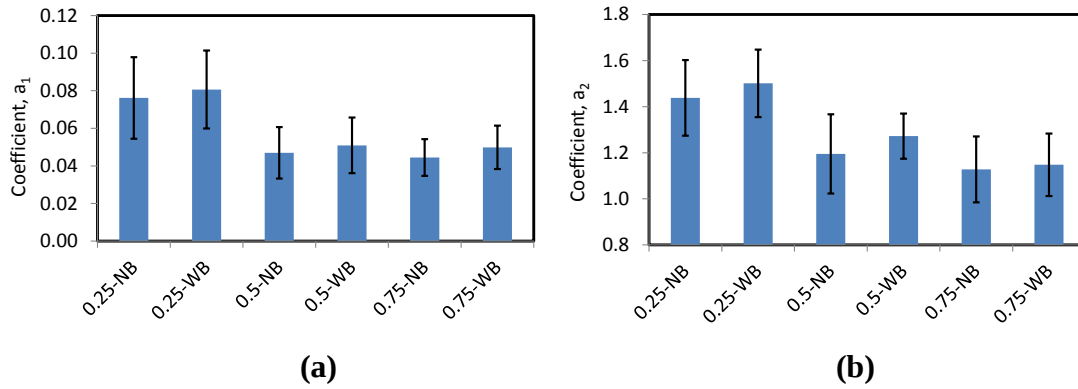
Figure 3.12: Mean and standard deviations of regression coefficients corresponding to each sitting posture and excitation condition: (a) a_1 ; (b) a_2 .
