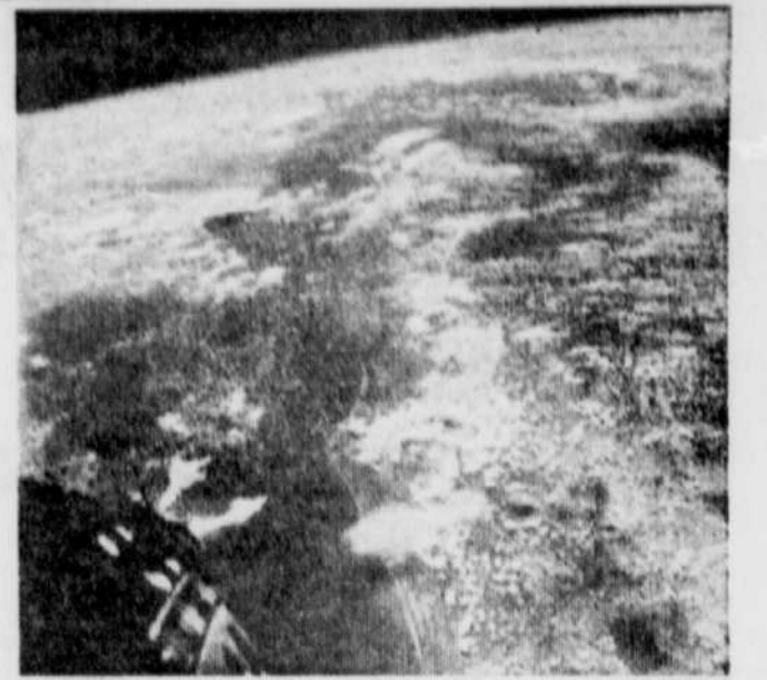
ASTRONAUTS' VIEW OF LAUNCH SITE — This photo taken by astronauts Gordon Cooper and Charles Conrad during the flight of the Gemini 5 shows the eastern coast of Florida and the Bahama Islands. Cape Kennedy is located on the tip of the bulge in the coastline and the Bahamas are located in upper left of photo under partial cloud cover. Part of the spacecraft is in lower left of photo (AP Wirephoto from NASA)
