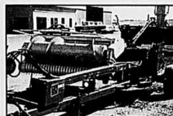
Fourragère John Deere 3960, pick-up, nez 2 rangs. Stanbridge. P.S.D.
