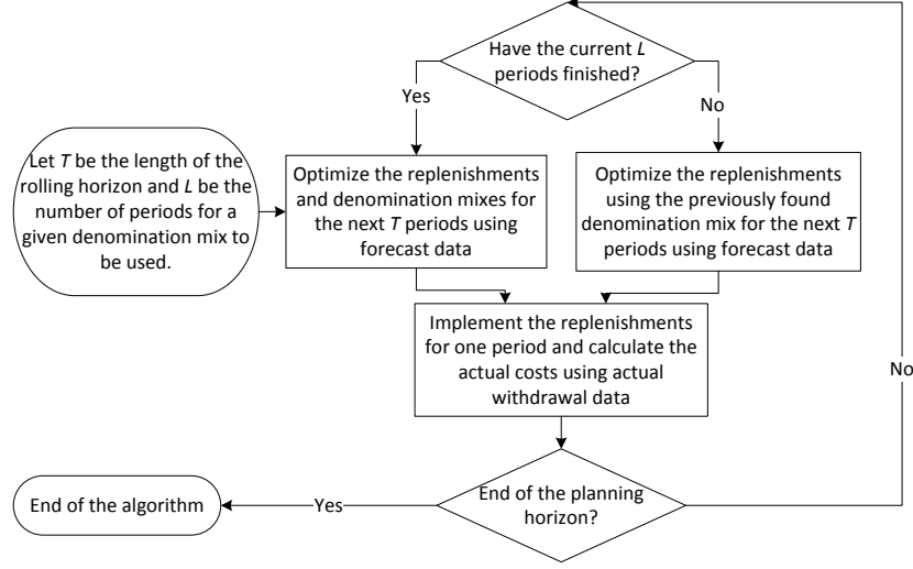
Figure 1: Overall scheme of the time-varying algorithm
