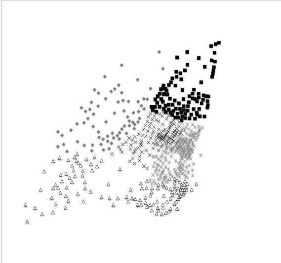
(a) |R| = 5
