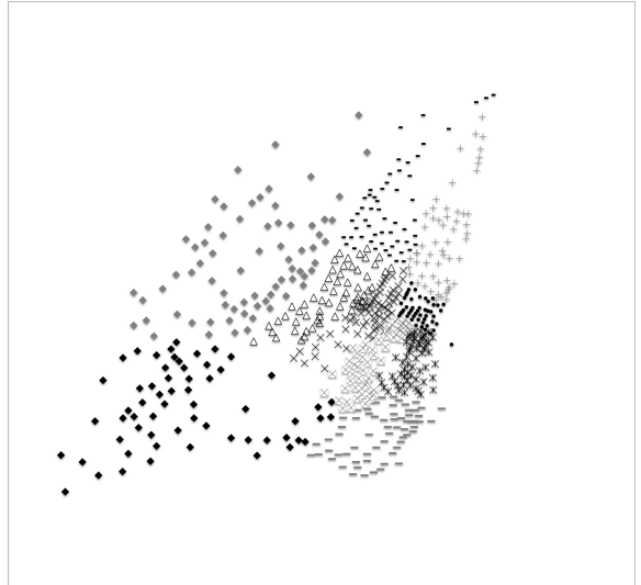
(c) |R| = 15
