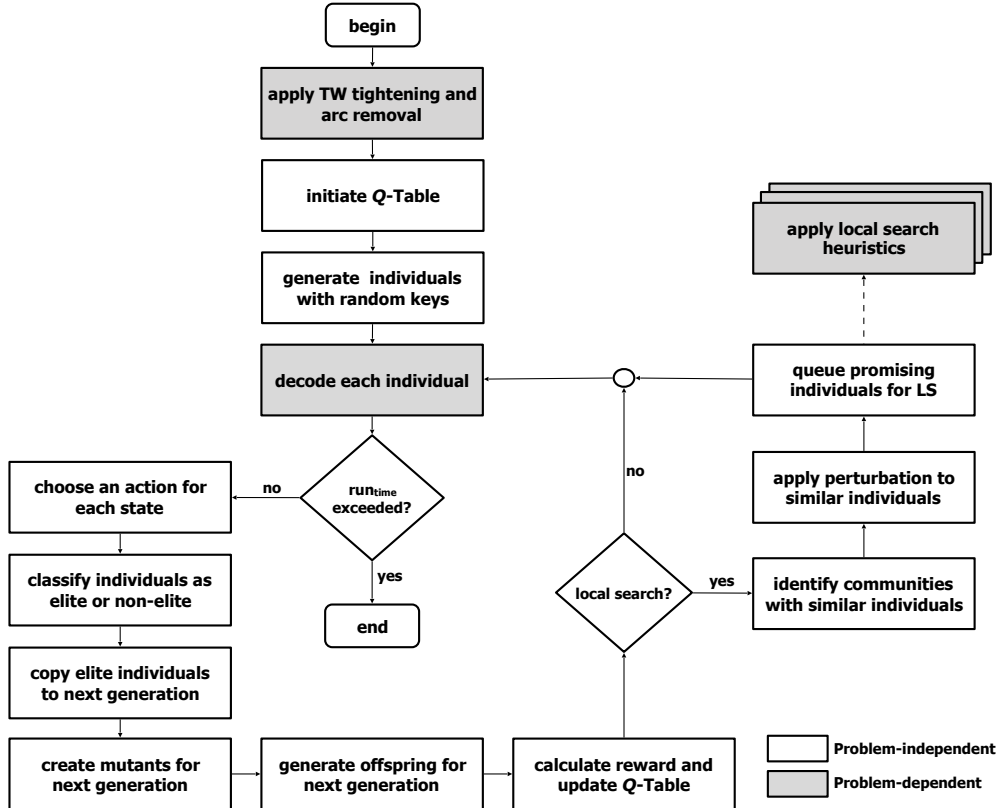
Figure 2: BRKGA-QL scheme
