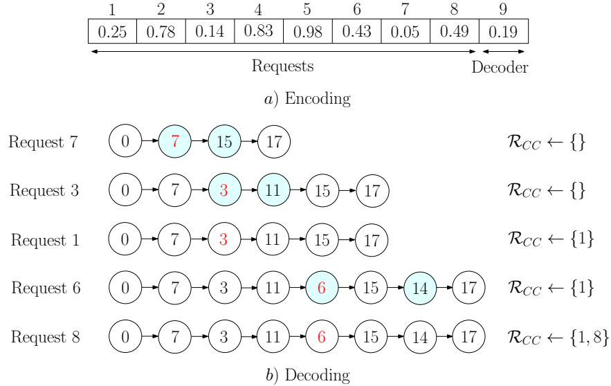
Figure 1: Encoding and decoding process
