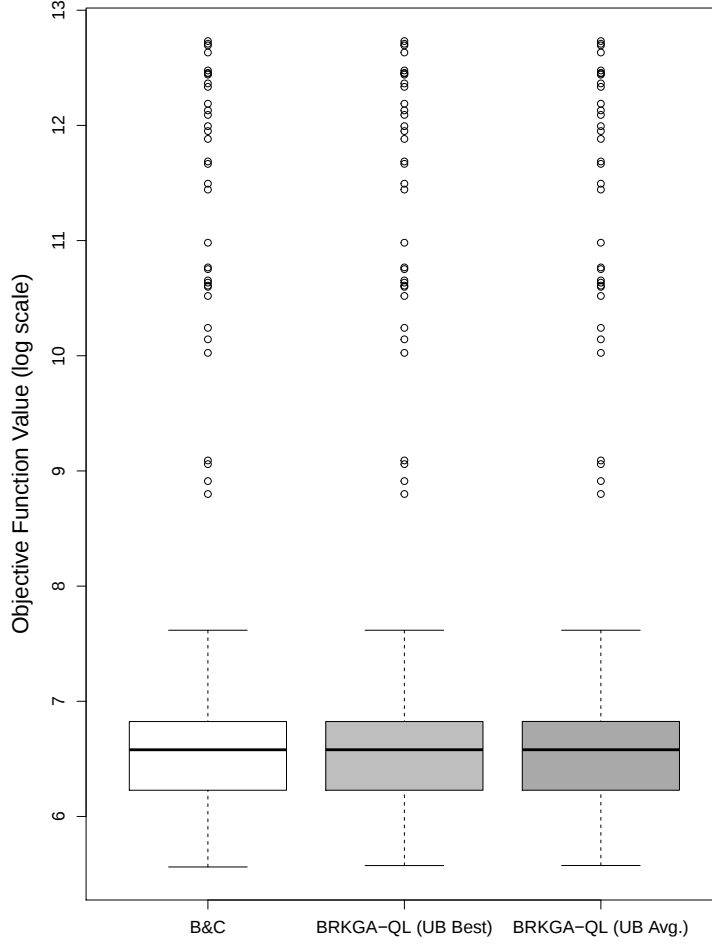
Figure 3: Boxplot with solution costs found by B&C and BRKGA-QL (best and average upper bounds).
