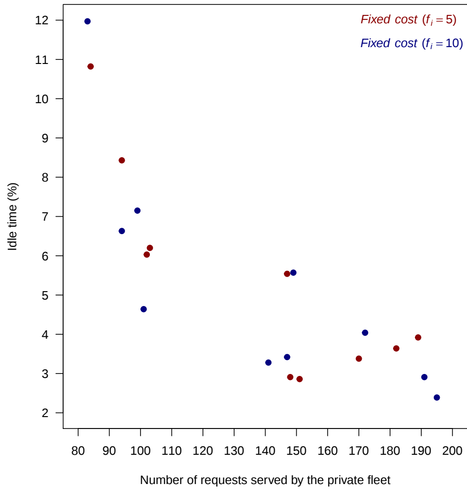
Figure 4: Idle time of the private fleet
