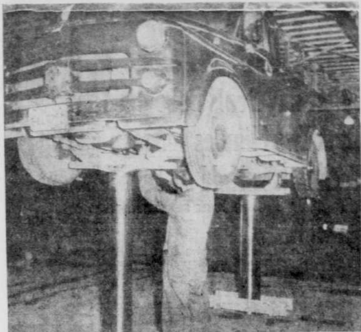
After a day on the road, Bell company repair trucks return each evening to the company's work centre on 10th avenue where they are serviced, washed down and restocked with equipment, ready to take the road again the following morning. Shown above, Norman Lefebvre, a company mechanic, is preparing to change the oil of a repair truck in the workshop section of the garage.
