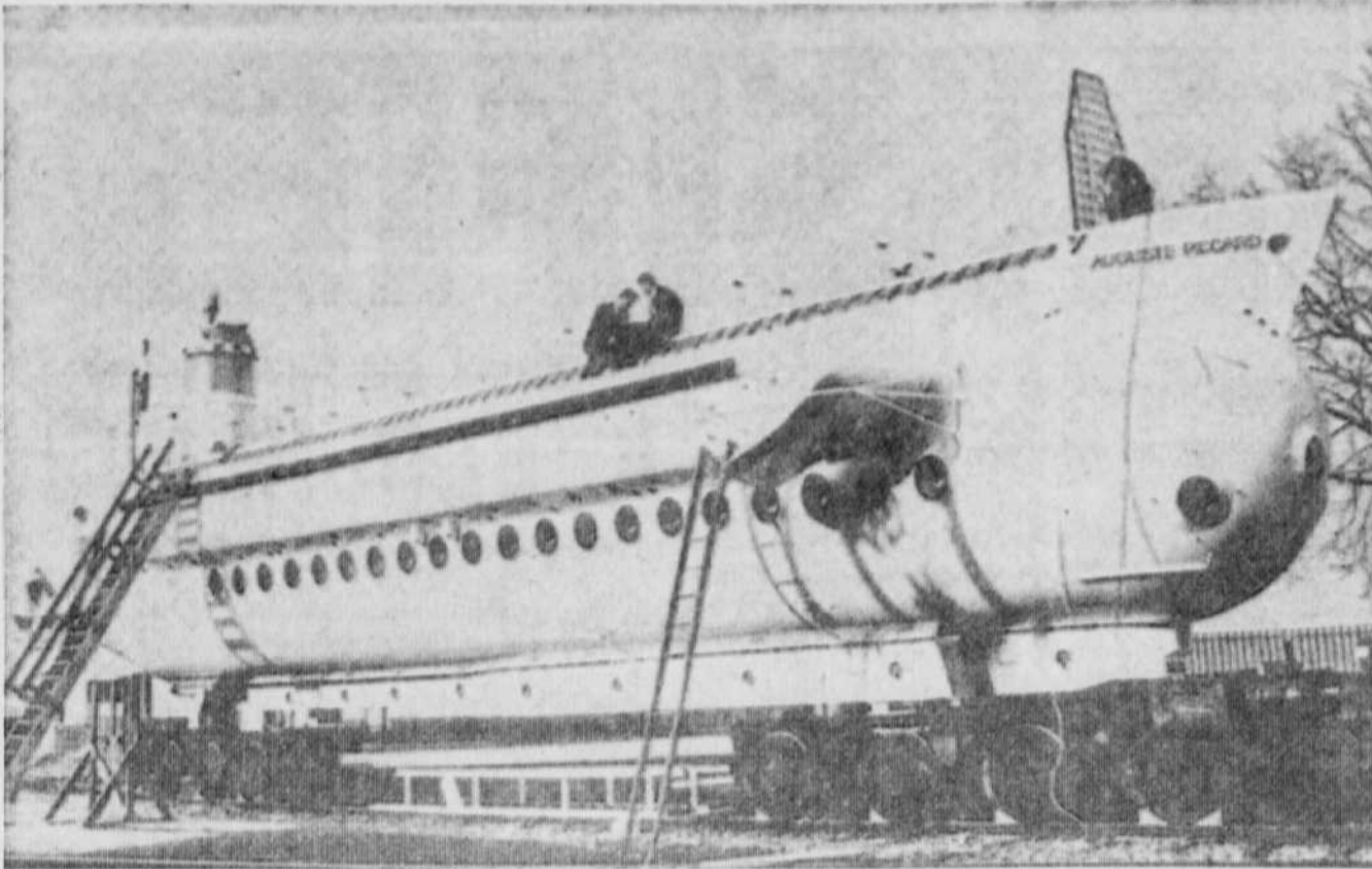
SUBMARINE FOR GULF STREAM STUDY — Dr. Jacques Picard plans to use this 93-foot research submarine on an estimated six weeks cruise drifting with the Gulf Stream from Florida to Newfoundland. One aim of the cruise is to determine if defense problems along the coast involves the underwater continental shelf. The submarine, pictured on railroad wheels, has operated in the depths of Switzerland's Lake Geneva, but has not yet been brought to this continent. (AP Wirephoto)
