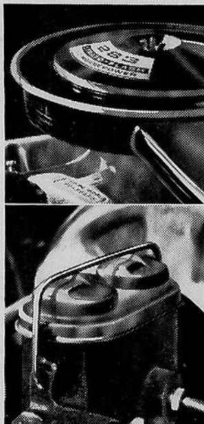
Grande Parisienne's standard engine is a 195 hp V8. Optional V8s have horsepower ratings of 275, 325 and 385. The twin-domed affair is Pontiac's dual master cylinder, heart of its new brake system.
