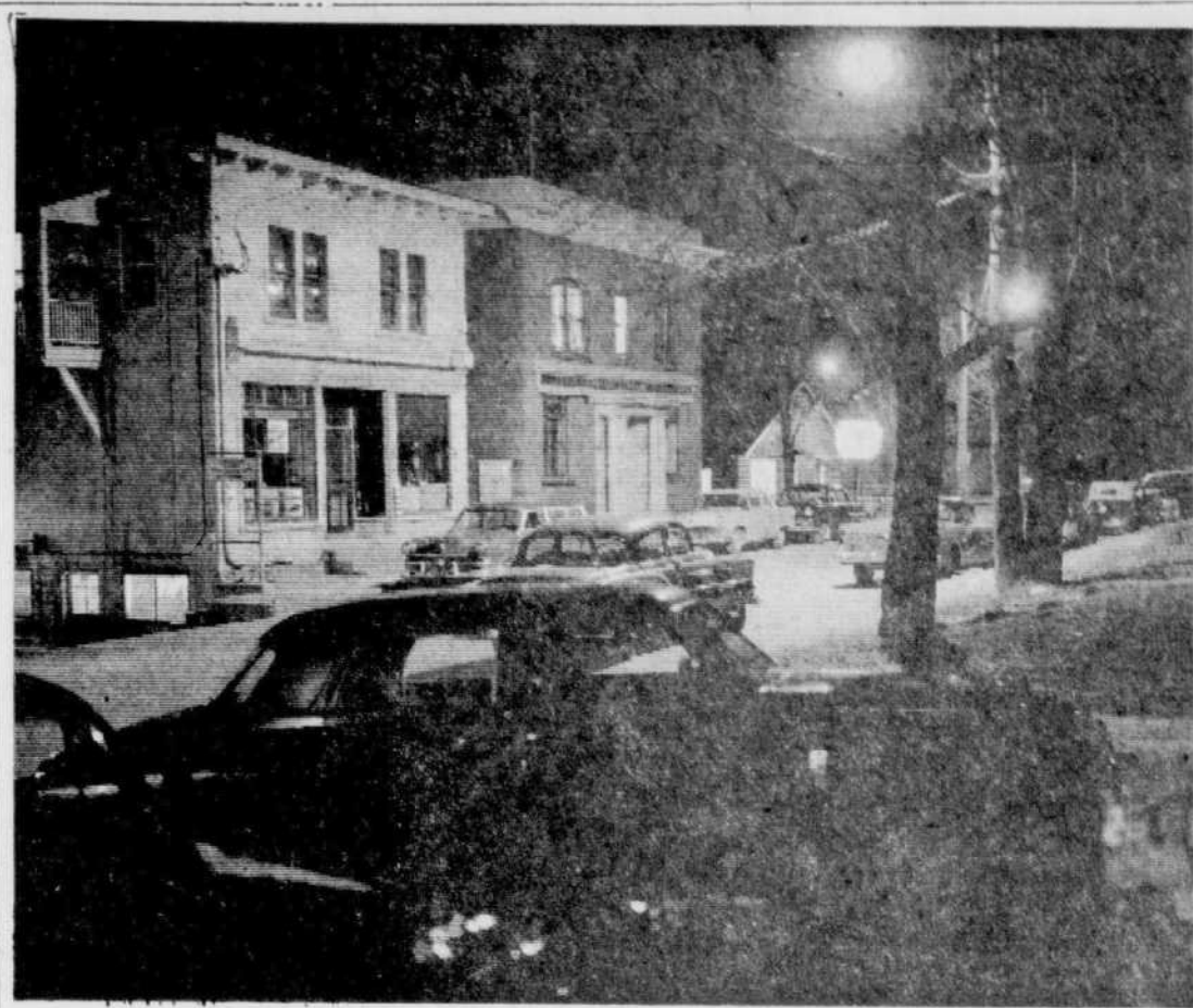
NIGHT OR DAY? — Installation of the new lighting system on Main Street in North Hatley makes it hard to tell which it is. The old 200-watt incandescent lamps which had a life expectancy of three months have been replaced with 400-watt mercury vapor lamps which last two years. Cost of individual lamps is higher, but overall cost is about the same.
