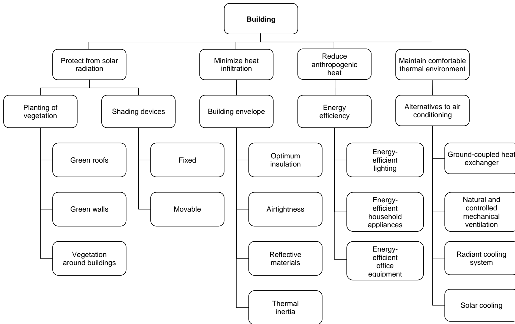
Figure 10 Schematic diagram of urban heat island mitigation strategies involving buildings
