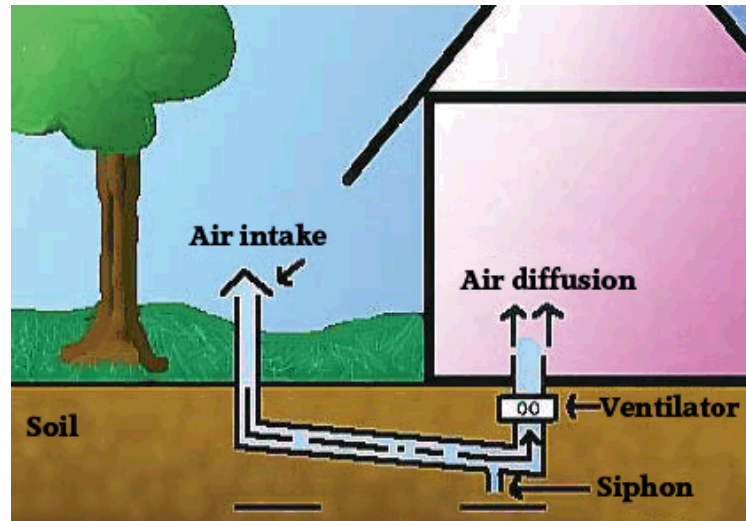
Figure 9 Cross-section of a ground-coupled heat exchanger
