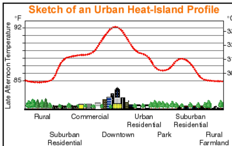
Figure 1 Sketch of an Urban Heat Island Profile
