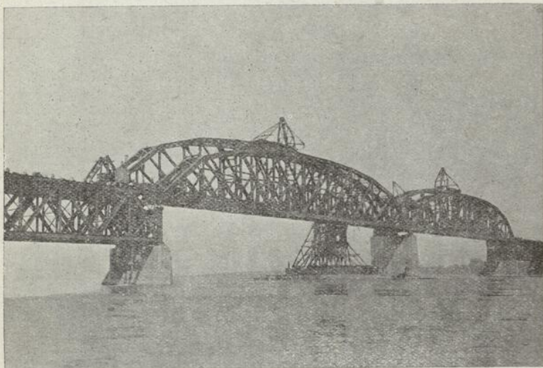
Bridge over the St-Lawrence River at Lachine, P. Q.
