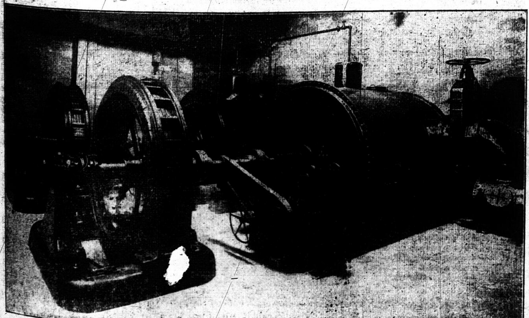
FIG. 3—VIEW OF WATERWHEELS, GOVERNORS AND GENERATORS.
