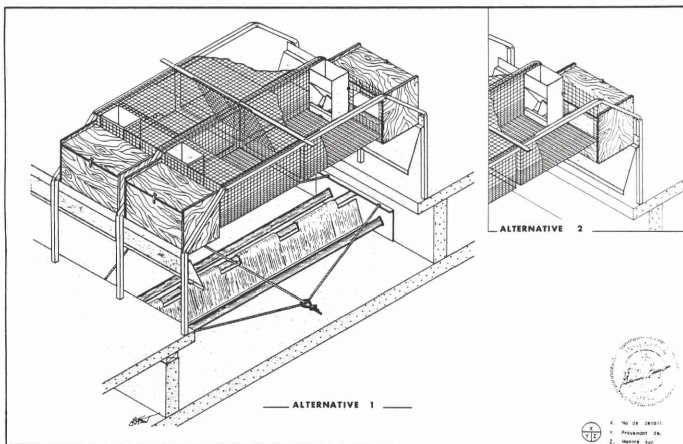
FIGURE 4 CAGE DE MISE-BAS
