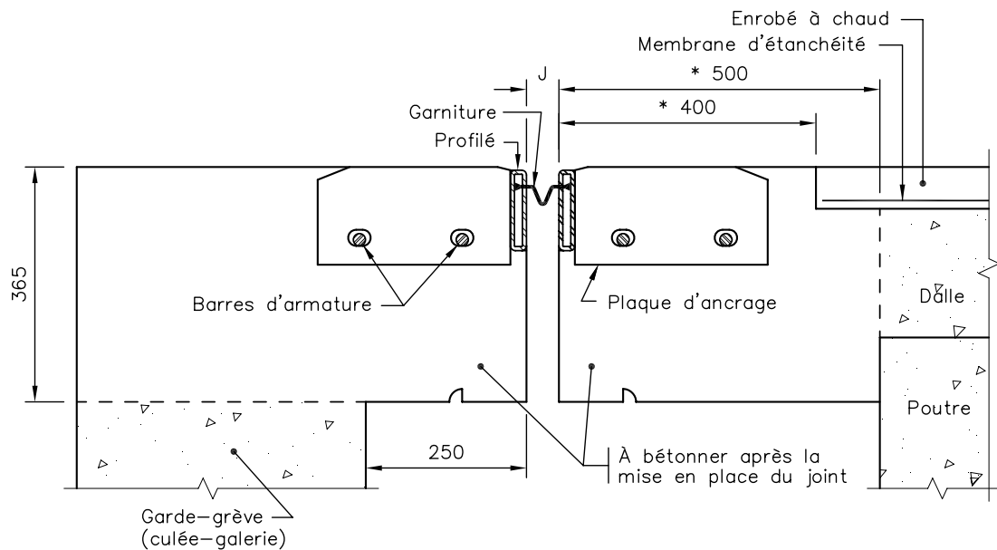
JOINT DE TABLIER HSS
