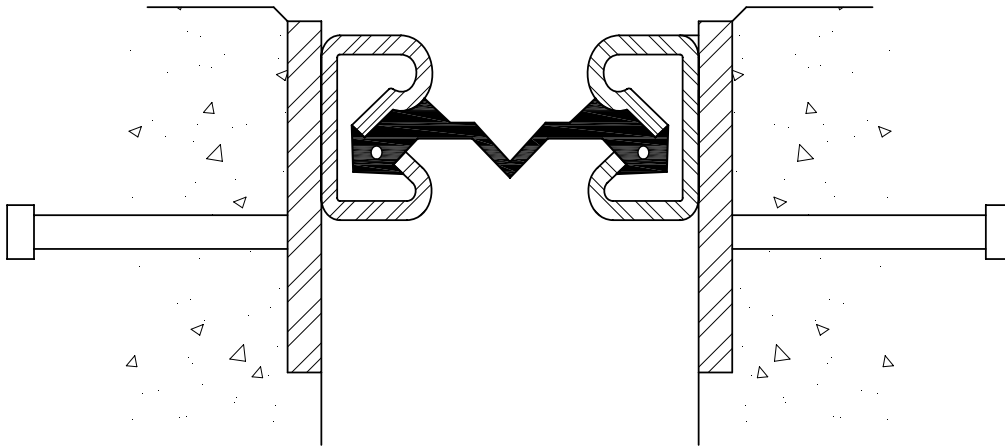
Figure 11.3-15 Joint longitudinal
