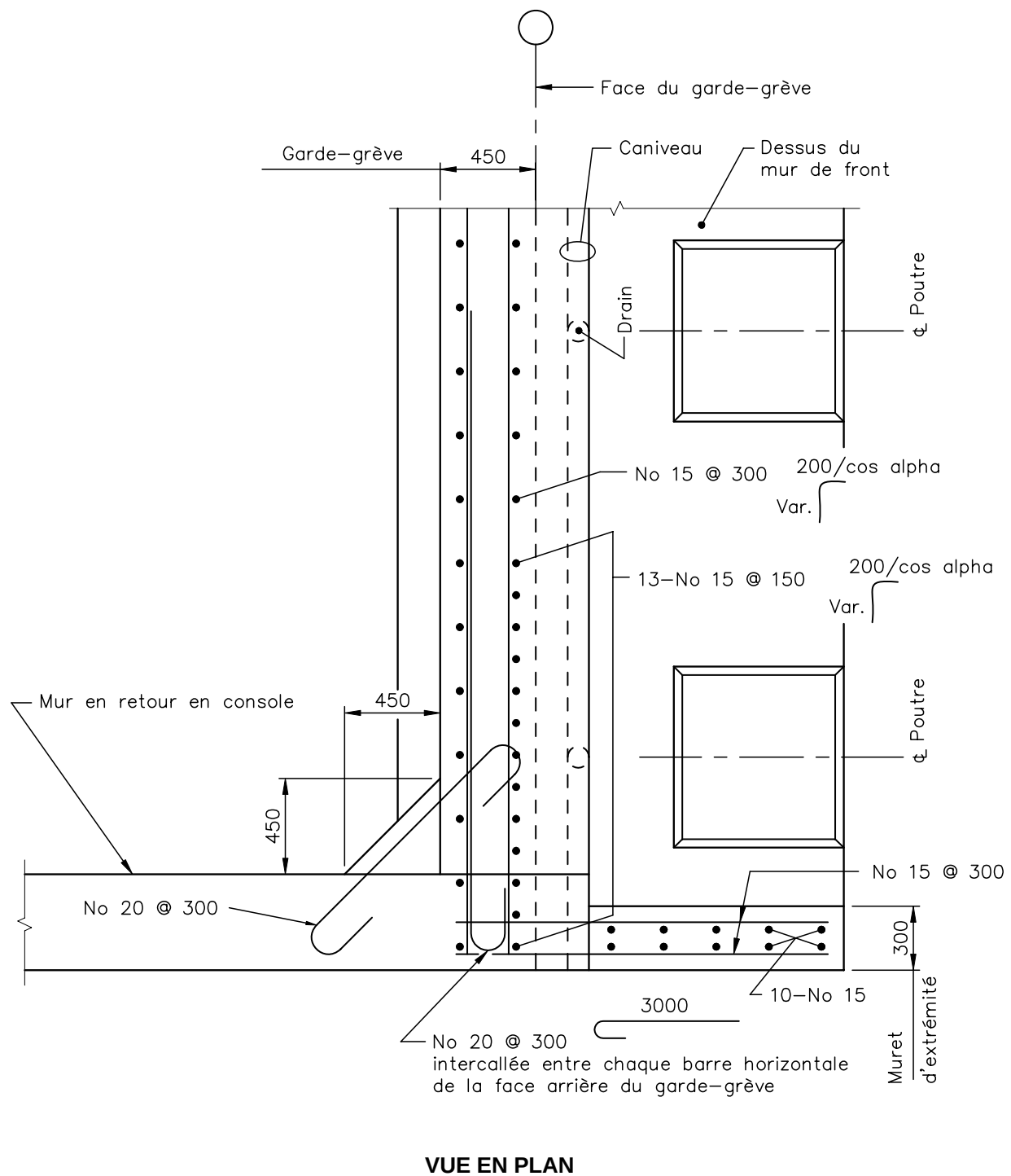
Figure 11.3-8 Culée-galerie (armature – suite 2)
