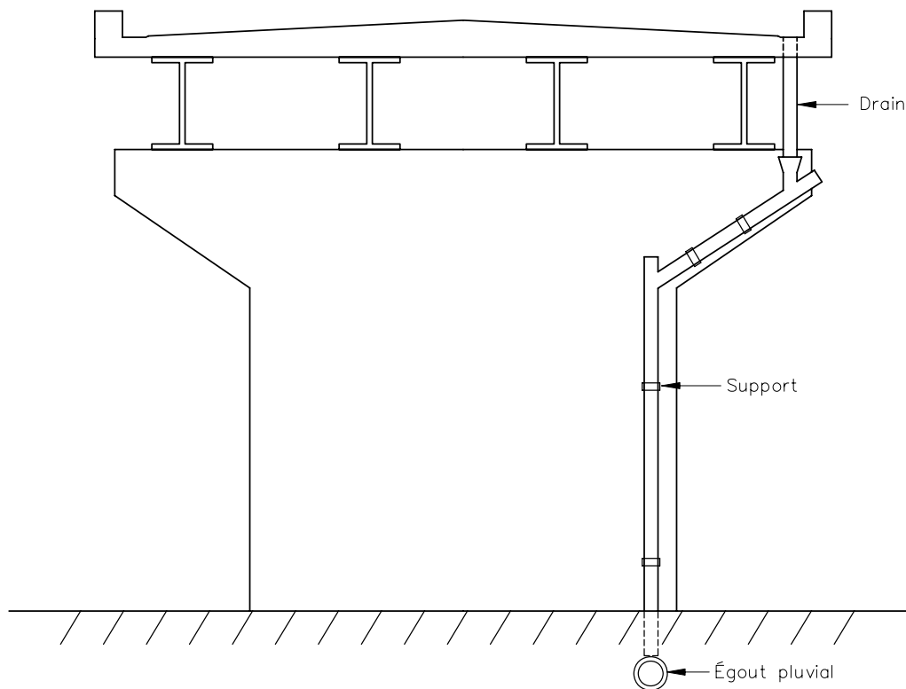
Figure 2.2-3 Tuyau de descente
