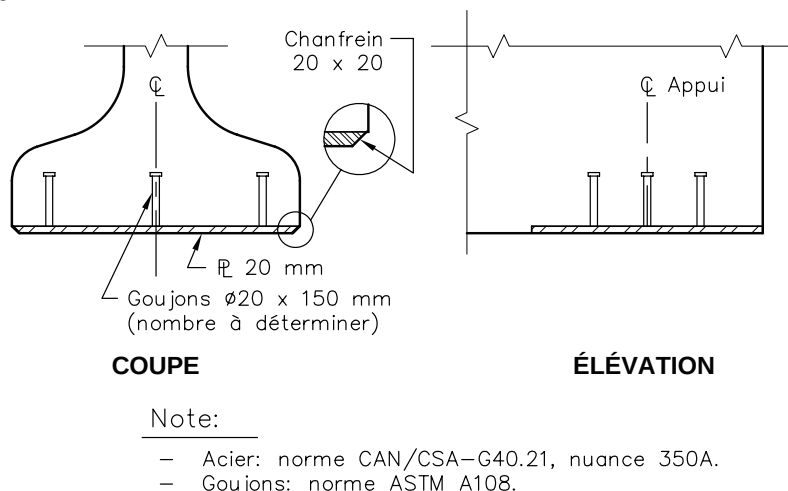
Figure 8.3-18 Plaque d'ancrage
