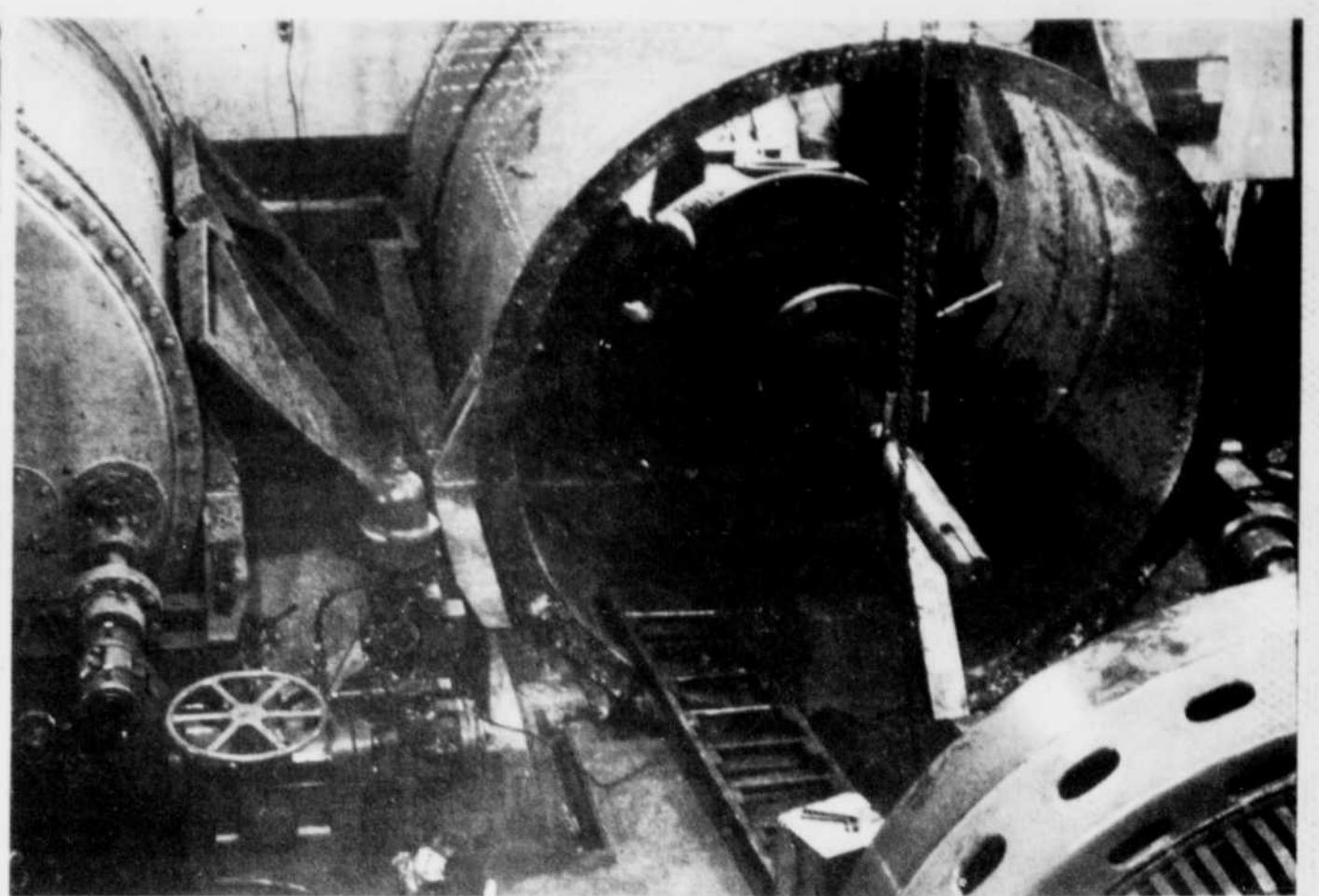
One of the huge turbines of Frontenac Dam is seen under repair. When fixed, water rushing into it turns the propeller which creates electricity in the generator.
