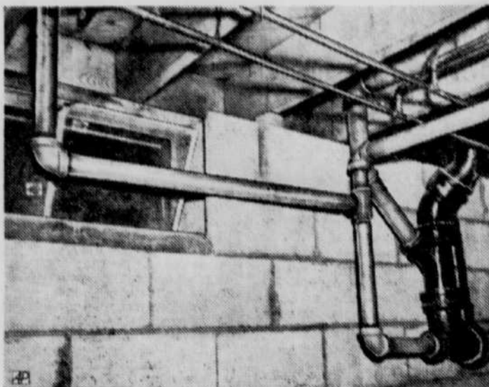
CARELESS planning was responsible for this bad plumbing job. Notice the sharp elbows inviting drainage trouble and the placement of a drain pipe where you can't open cellar window.
