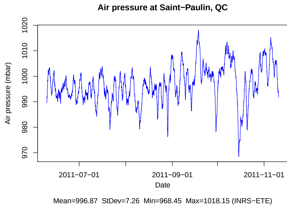
Figure 2.12: Air pressure.
