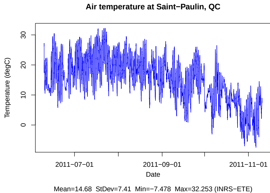
Figure 2.9: Air temperature.
