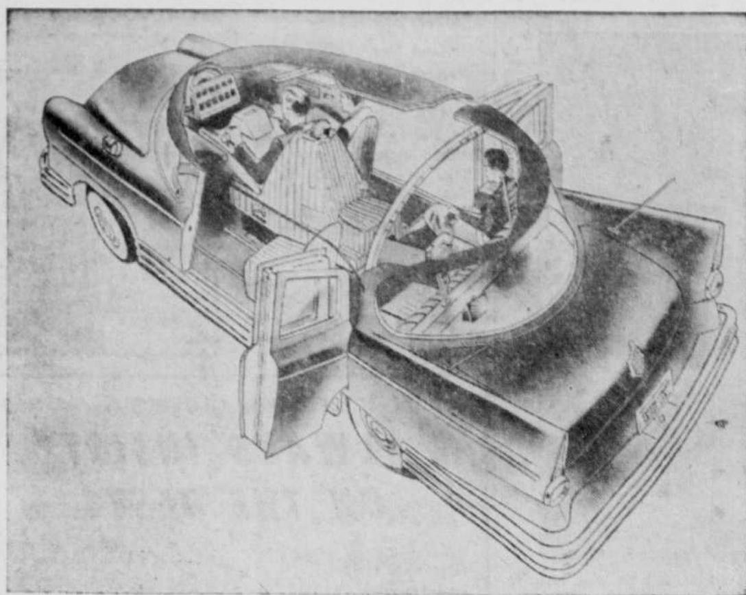
DESIGN FOR SURVIVAL — Shown above is the result of five years' study of auto crashes by Cornell Aeronautical Laboratory of Buffalo and Liberty Mutual Insurance Co. of Boston. Designed with the sole aim of eliminating the major causes of passenger injuries and fatalities in smashups, the car affords maximum safety to its occupants without sacrificing exterior styling. Innovations include centrally seated driver, lever system to replace steering wheel and column, padding, seat belts or yokes and roll-over bars above passengers. Note one "club-car" seat facing rear. Outside, shock-absorbing material is sandwiched between the bumpers. Telephone booth-type doors and reinforced frame prevent cave-ins of the sides in collisions.
