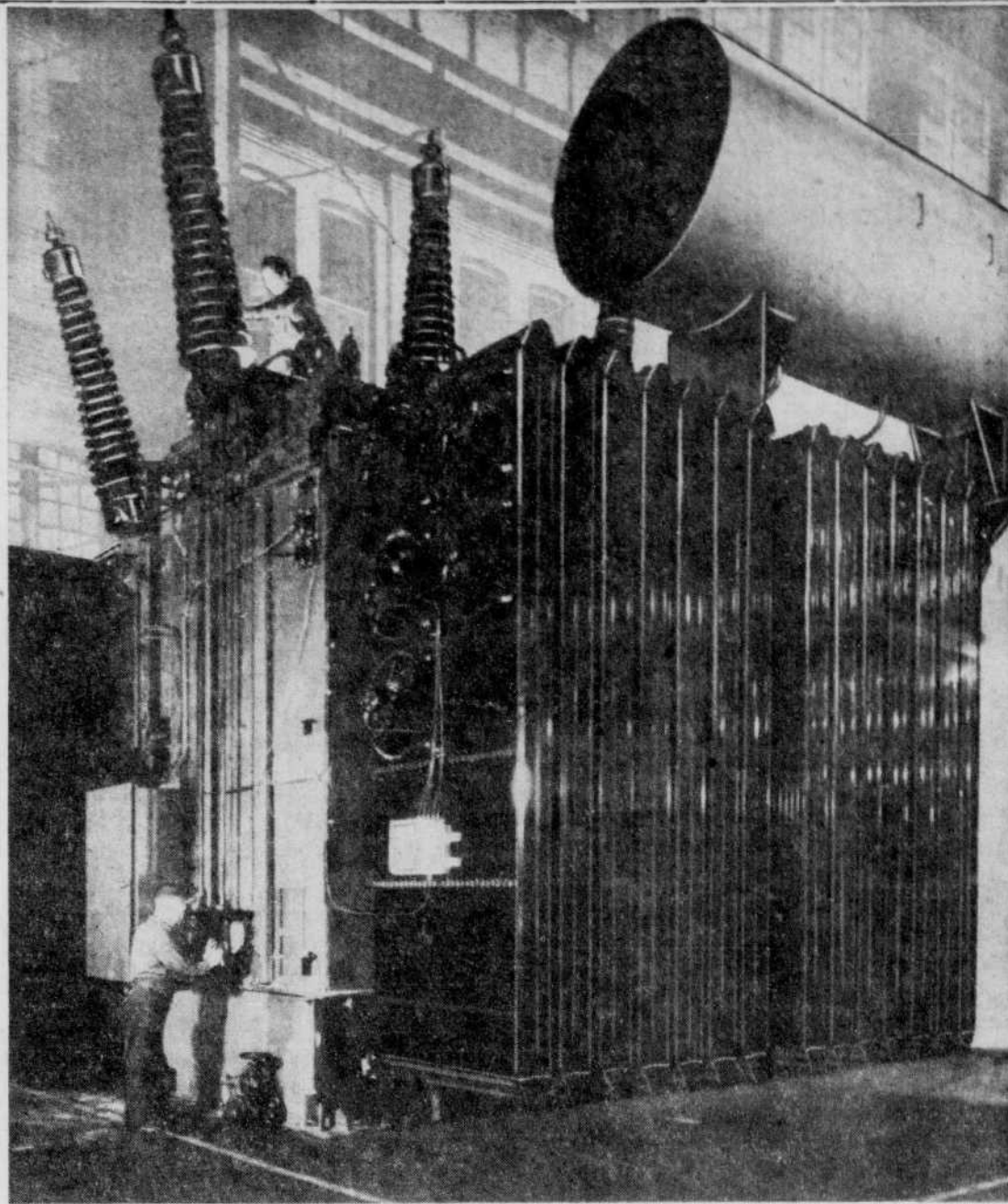
A Power Giant — This huge power transformer just completed at Canadian Westinghouse in Hamilton for the Quebec Hydro's vast Bersimis power project is capable of staggering power production. It weighs over 325 tons, stands as high as a normal house and contains enough fuel oil to heat an average six-room home for 30 years. Its power is enough to light 2½ million 60 watt lamps, or, if you want to go into the subject even more, it is capable of producing light to street lamps spaced at a hundred feet apart right around the earth at the equator. This one will be installed at Charlesbourg, near Quebec City, this year. Others will be installed near Montreal. (Photo by Fed News)
