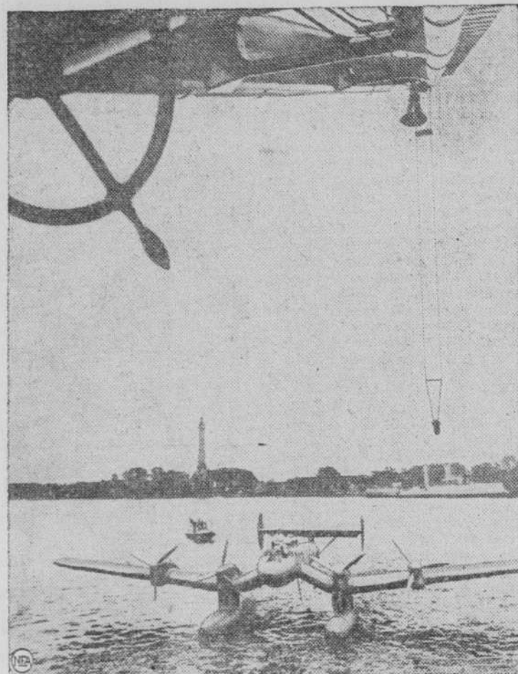
Floating air bases in midocean are being tested by the Luftwansa, German airplane company, for use as service and refueling stations on its North Atlantic commercial service. The "Friesenland," largest of four vessels to be used for that purpose, is shown in the top picture. Giant cranes, such as pictured below, will be part of the floating "island" equipment, enabling the ships to lift the huge transport planes out of the water and onto the deck for inspection.
