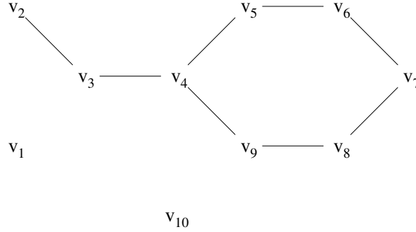
Figure 4: Partition found by HTREE ( s \geq 8 )
