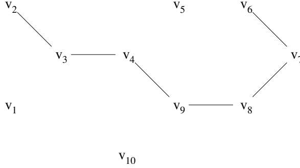
Figure 5: Optimal partition with maximum number of clusters ( s \geq 8 )
