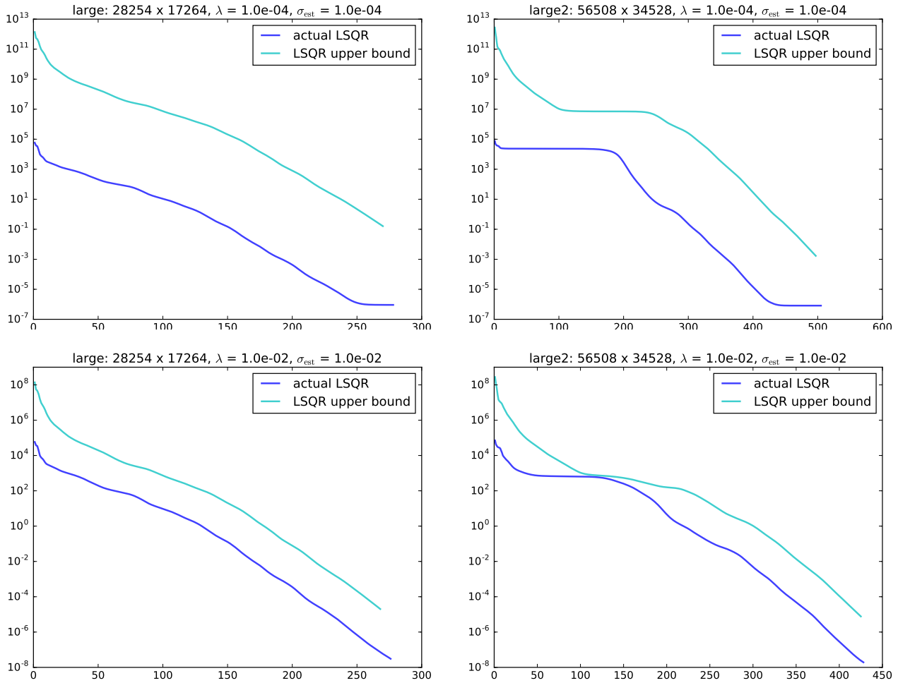
Figure 4: Error along the LSQR iterations on problems large and large2 with regularization. The cyan curve shows the upper bounds for \sigma_{\text{est}} = 1.0\text{e-}4 (top) and \sigma_{\text{est}} = 1.0\text{e-}2 (bottom).
