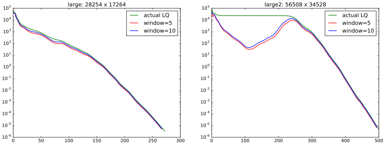
Figure 2: Error along the LSLQ iterations on problems large and large2 from the animal breeding set. The red and blue curves show the lower bounds with d = 5 and d = 10 .
