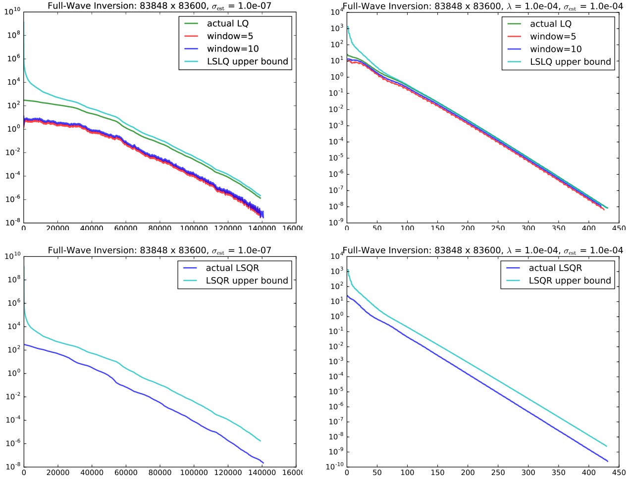
Figure 6: Error along the LSLQ and LSQR iterations on the seismic inverse problem without regularization (left) and with regularization (right).
