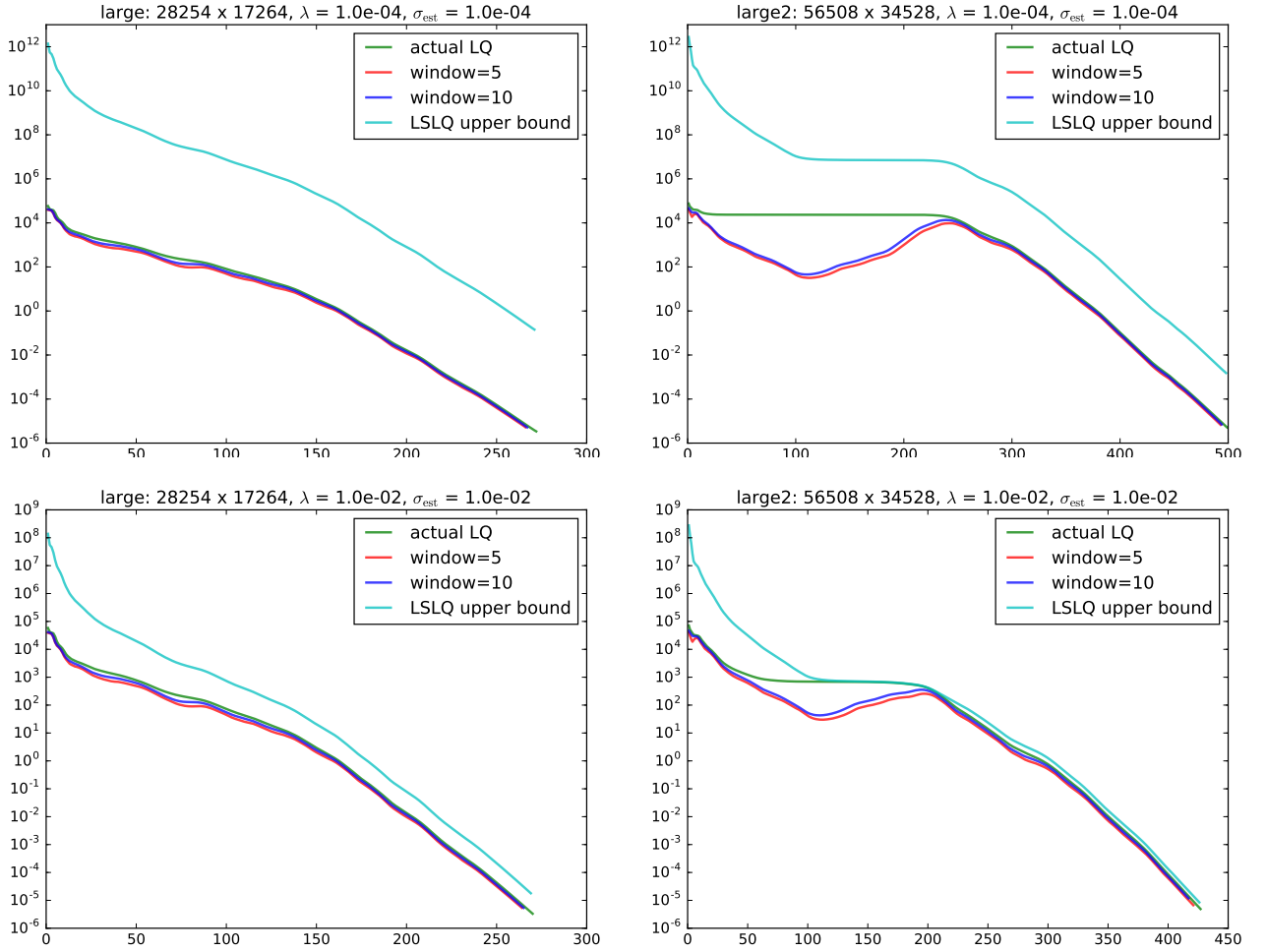
Figure 3: Error along the LSLQ iterations on problems large and large2 with regularization. The red and blue curves show the lower bounds with d = 5 and d = 10 . The cyan curve shows the upper bounds for \lambda = 1.0e-4 (top) and \lambda = 1.0e-2 (bottom).
