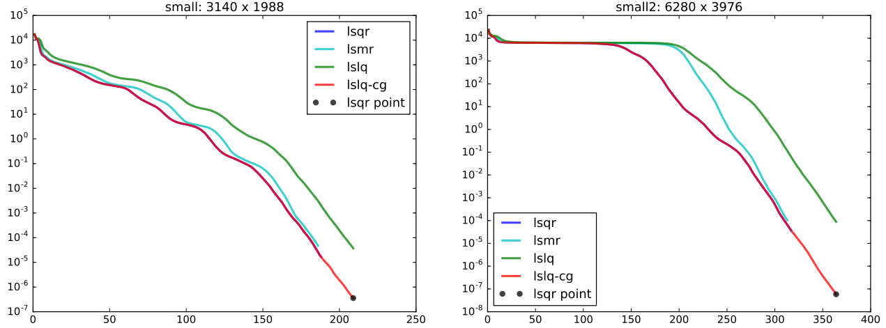
Figure 1: Error along the LSQR, LSMR and LSLQ iterations on problems small and small2 from the animal breeding set. The red curve corresponds to the LSQR iterates generated as a by-product during the LSLQ iterations. The horizontal axis represents the number of products with A and A^T .
