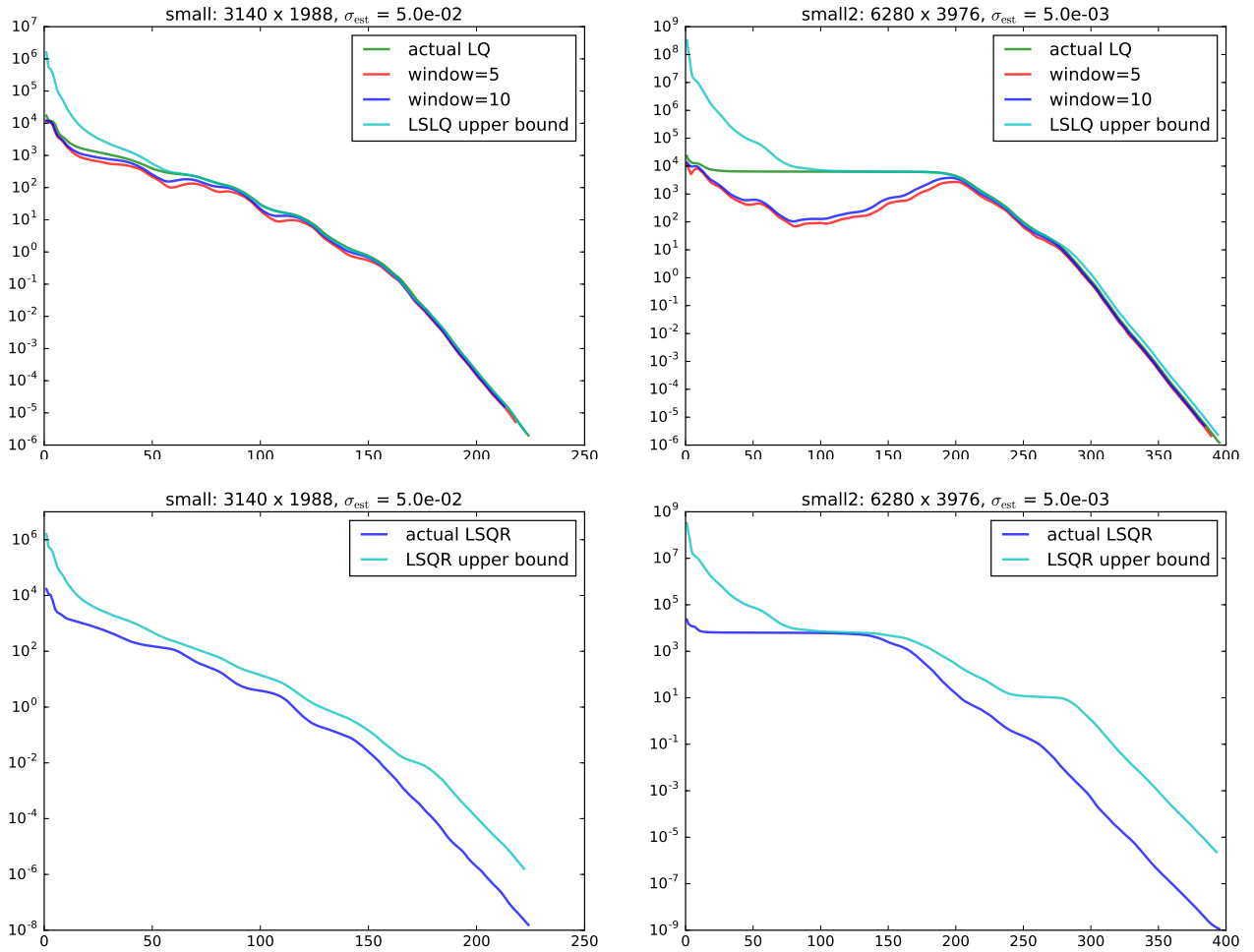
Figure 5: Error along the LSLQ and LSQR iterations on problems small and small2 without regularization. Both problems have rank-deficiency 1.
